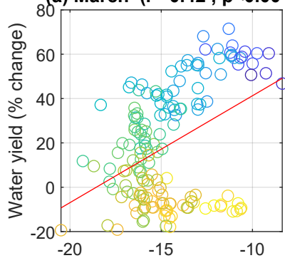
(a) March ( r = 0.42 , p < 0.001 )
