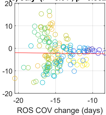
(e) July ( r = -0.01 , p = 0.862 )
