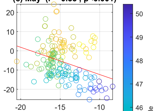
(c) May ( r = -0.33 , p < 0.001 )
