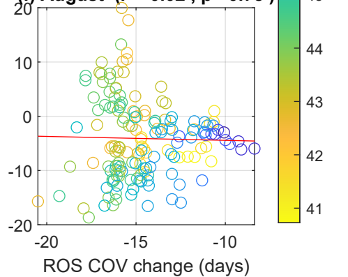
(f) August ( r = -0.02 , p = 0.78 )
