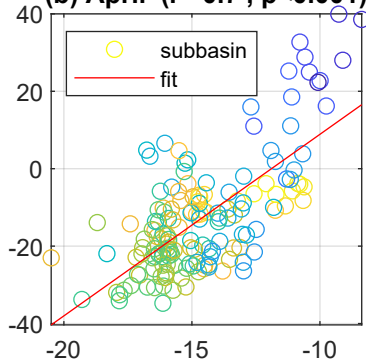
(b) April ( r = 0.7 , p < 0.001 )
