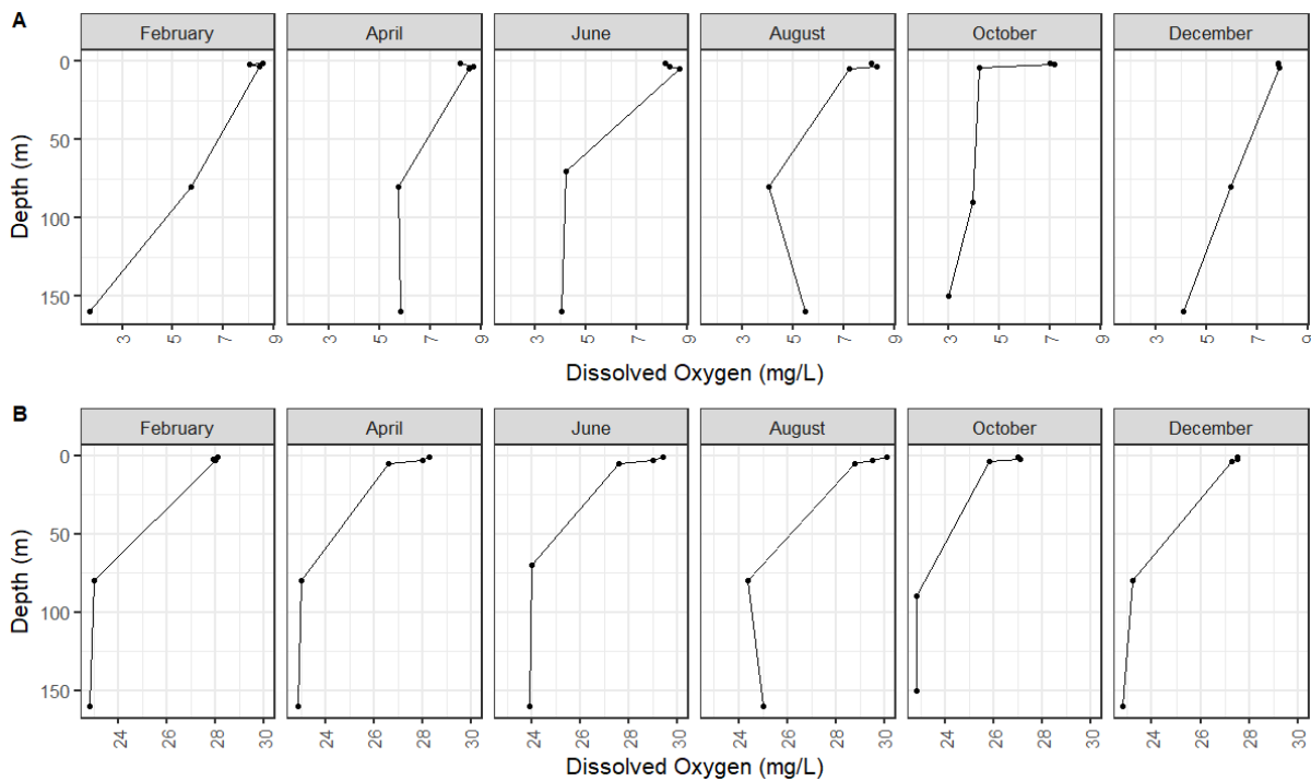
Fig. S2. Depth profiles of dissolved oxygen and temperature for La Miel Reservoir in Caldas, Colombia measured in 2018. Data source: Autoridad Nacional de Licencias Ambientales
