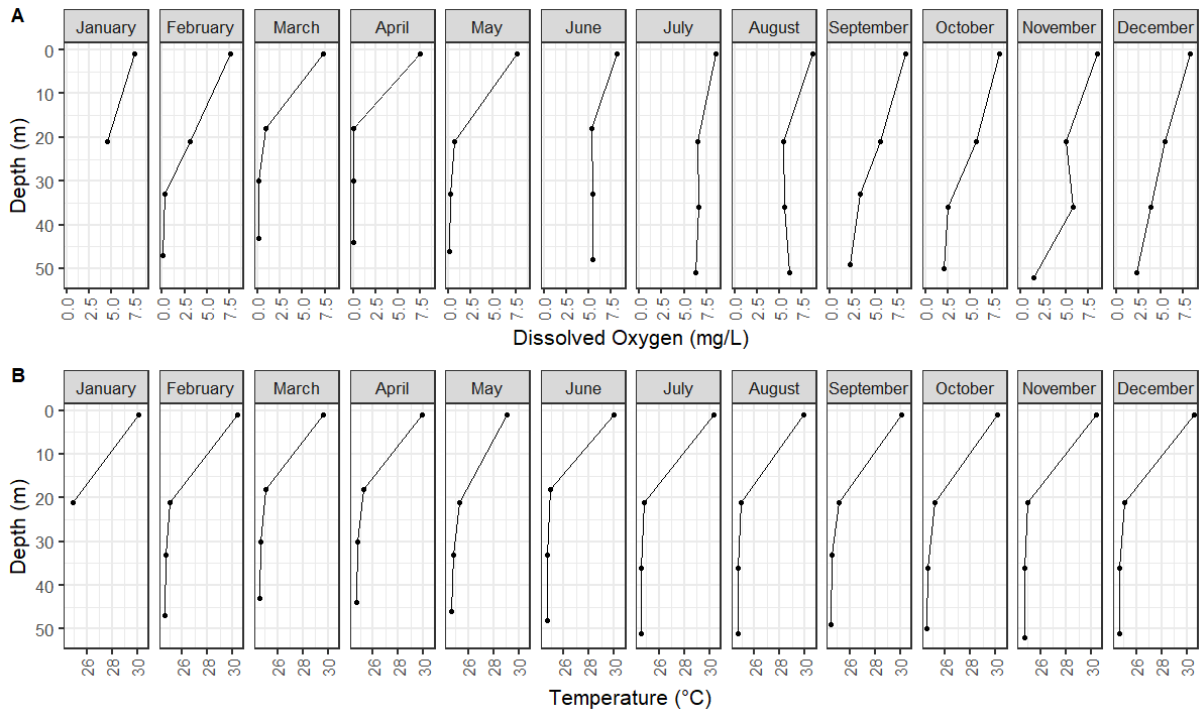
Fig. S1. Depth profiles of dissolved oxygen and temperature for Urra Reservoir in Cordoba, Colombia measured in 2018. Data source: Autoridad Nacional de Licencias Ambientales
