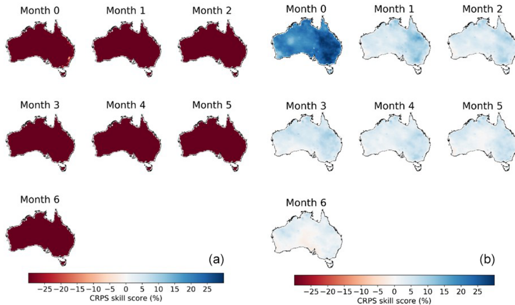
Figure 5. CRPS skill scores in (a) raw and (b) calibrated forecasts at seven lead times during 1990–2019.
