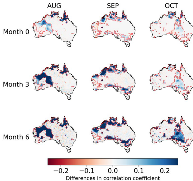
Figure 2. Differences in the correlation coefficient ( r ) between BJP-ti calibrated forecasts and observations with that between BJP calibrated forecasts and observations for 3 selected months (August, September, and October) and three lead times (months 0, 3, and 6). Red polygons show regions with significant observed trends.
