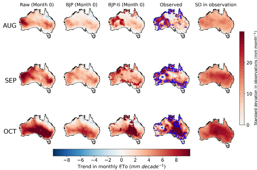
Figure 1. Trends in raw forecasts, BJP calibrated forecasts, and BJP-ti calibrated forecasts at month 0 and observed ET_0 in August, September, and October. Blue polygons show regions where observed trends are statistically significant. SD refers to the standard deviation.
