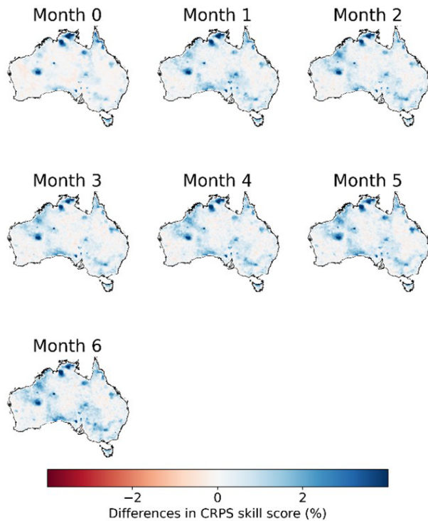
Figure 4. Differences in CRPS skill scores between BJP-ti calibrated forecasts and the BJP calibrated forecasts over 1990–2019.
