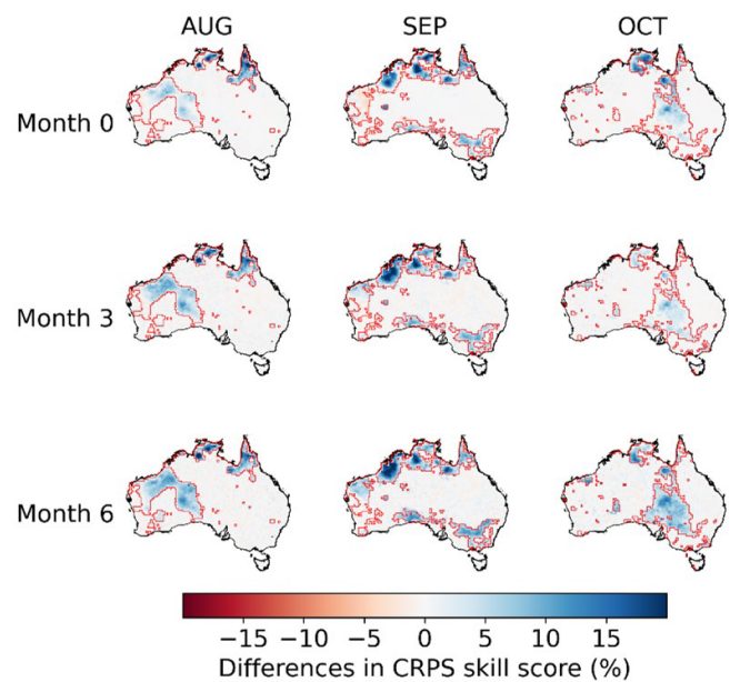
Figure 3. Differences in CRPS skill scores between BJP-ti calibrated forecasts and the BJP calibrated forecasts for 3 selected months (August, September, October) and three lead times (months 0, 3, and 6). Red polygons show regions with significant observed trends.
