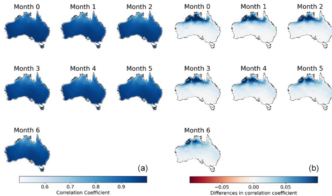
Figure 8. (a) Correlation coefficients between BJP-ti calibrated forecasts and observations and (b) improvements in correlation coefficients through the calibration with the BJP-ti model relative to those between raw forecasts and observations.
