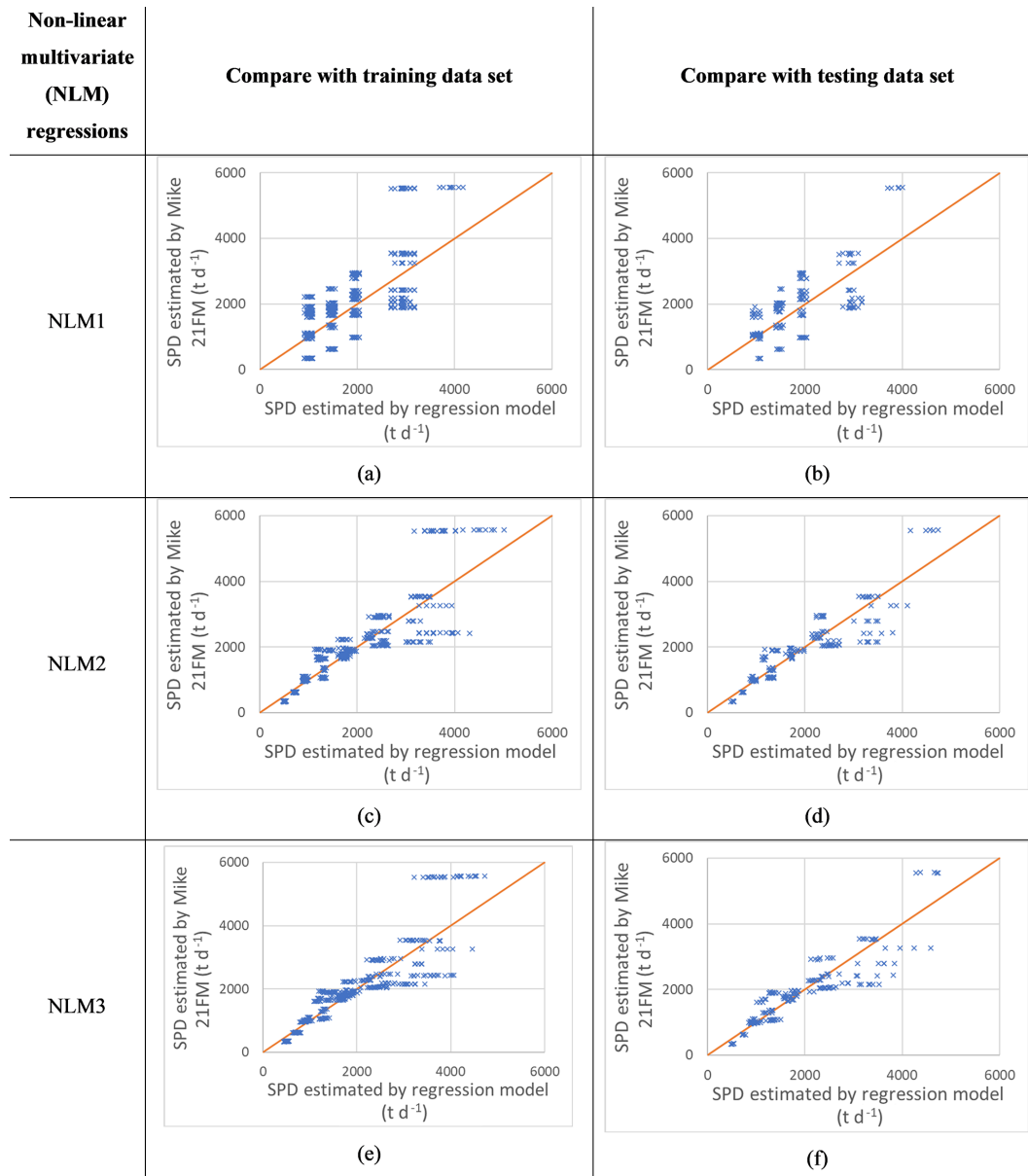
Figure 5. Comparing the values for SPD, calculated from the hydro-morphological model results against the values for SPD, estimated with the NLM regressions, for all 10 sets of training and testing data samples. The line depicts the 1 : 1 line.
