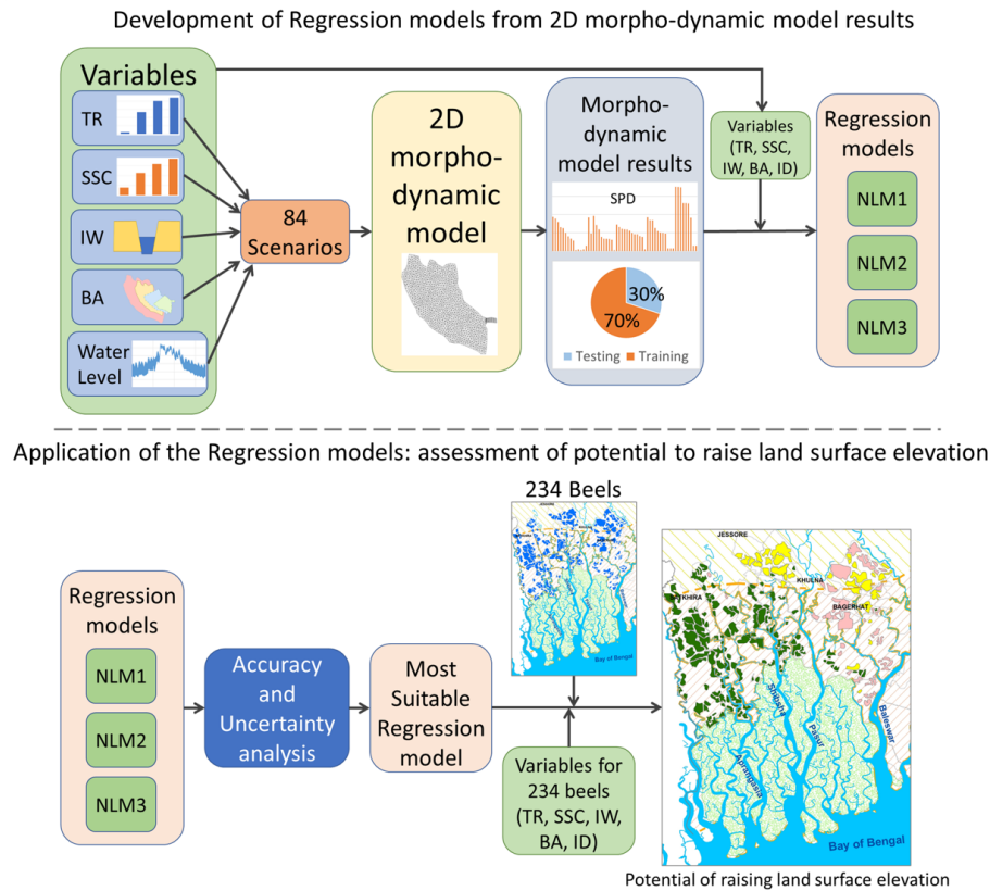
Figure 2. General approach used to establish the regression models for sediment deposition from physical control parameters and their subsequent application to estimate potential of raising land surface elevation throughout the southwestern Bangladesh delta.
