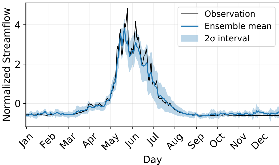
(a) GRANBY RIVER AT GRAND FORKS (08NN002) NSE = 0.87
