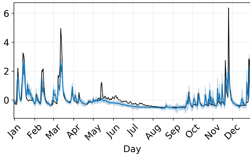
(b) ENGLISHMAN RIVER NEAR PARKSVILLE (08HB002) NSE = 0.59
