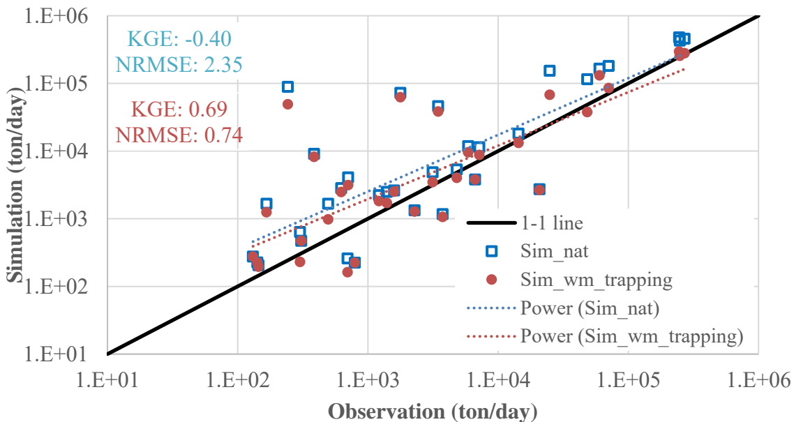
(b) Long-term average suspended sediment discharge
