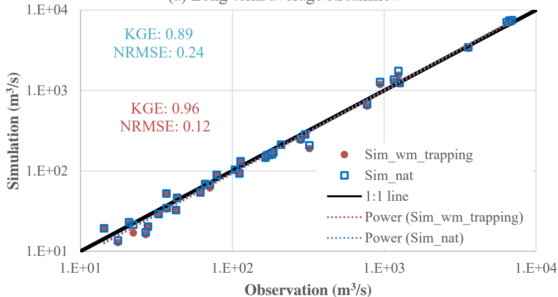
(a) Long-term average streamflow
