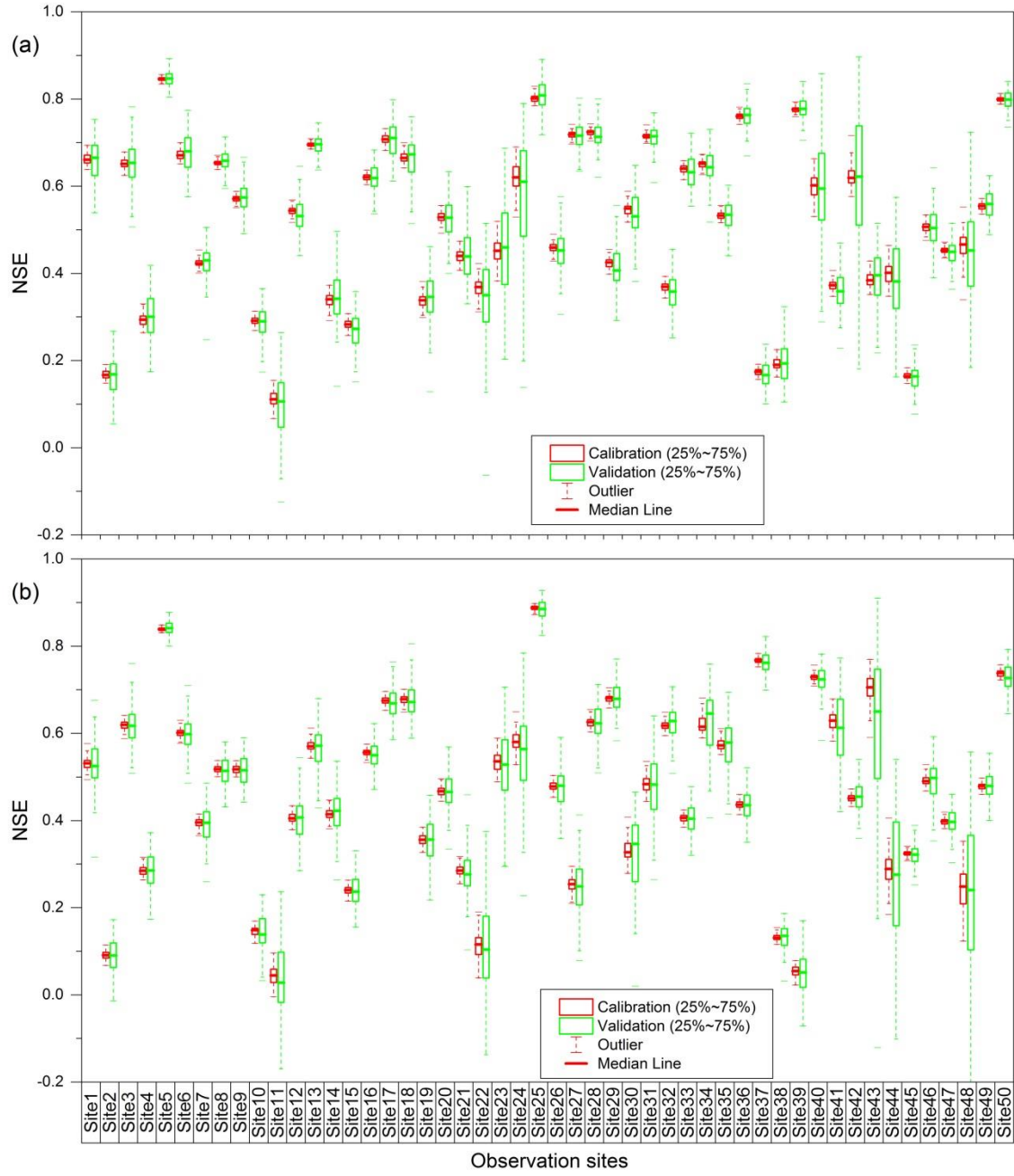
Figure S2: The performance of the LC_NDVI_P method in calibration and validation datasets at (a) 1030 and (b) 1330, respectively.
