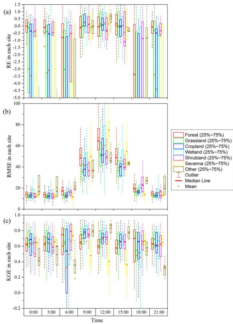
Figure S1: The RE, RMSE and KGE simulated by the LC method in each land cover type.
