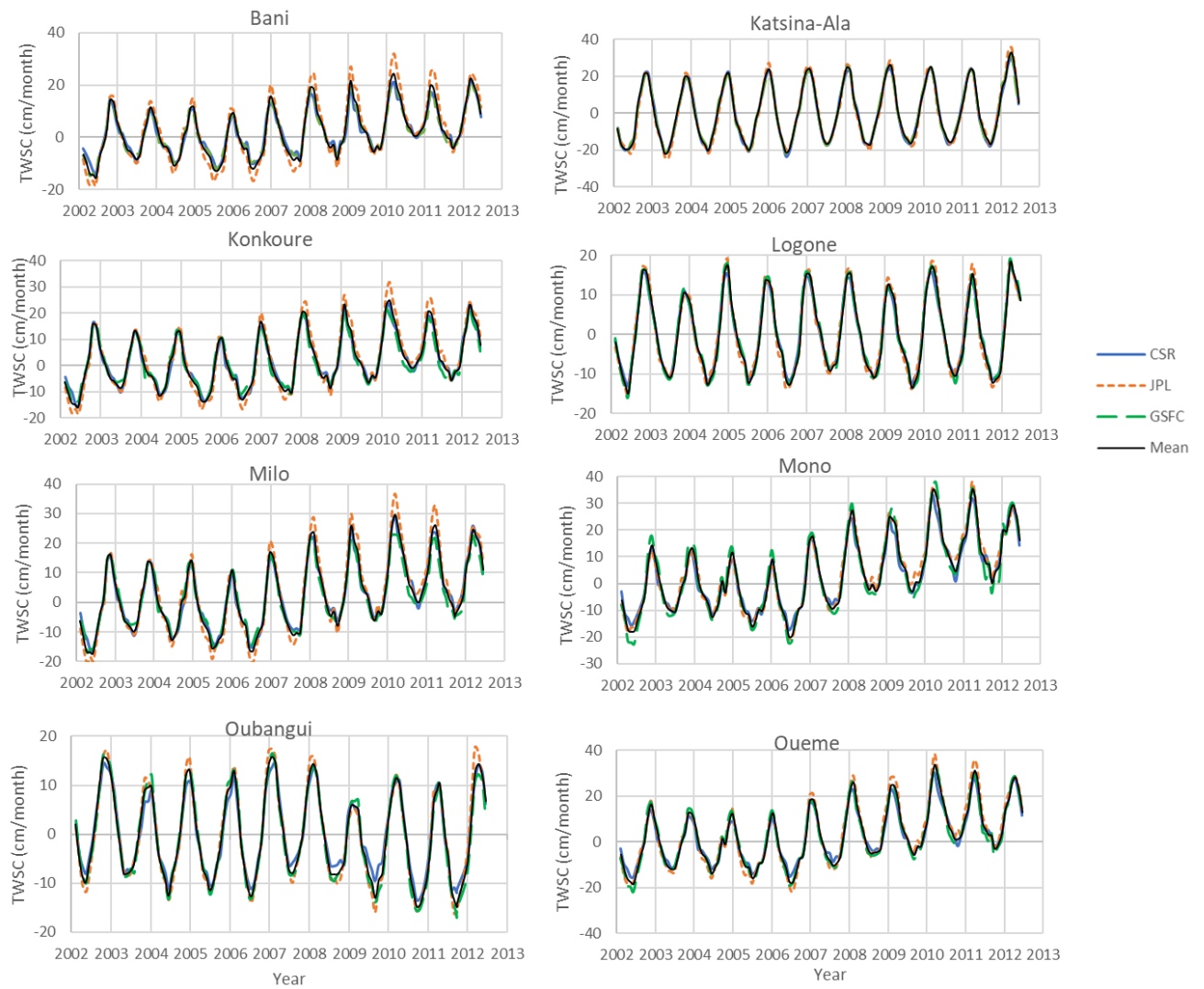
Figure S2: GRACE estimates from CSR, JPL, GSFC and their ensemble mean used in the study
