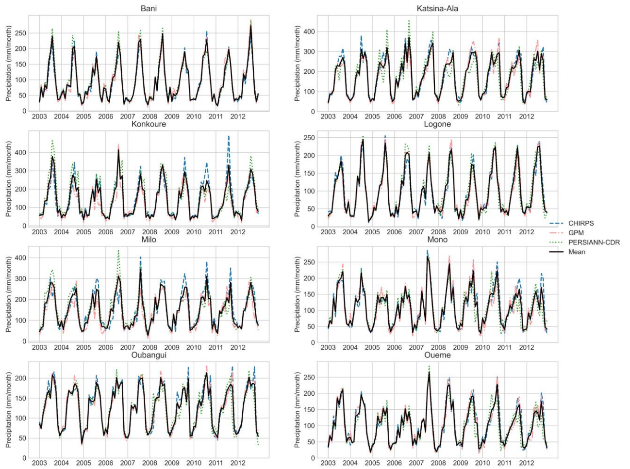
Figure S1: Precipitation Estimates from CHIRPS, GPM, PERSIANN-CDR, and their ensemble mean used in the study
