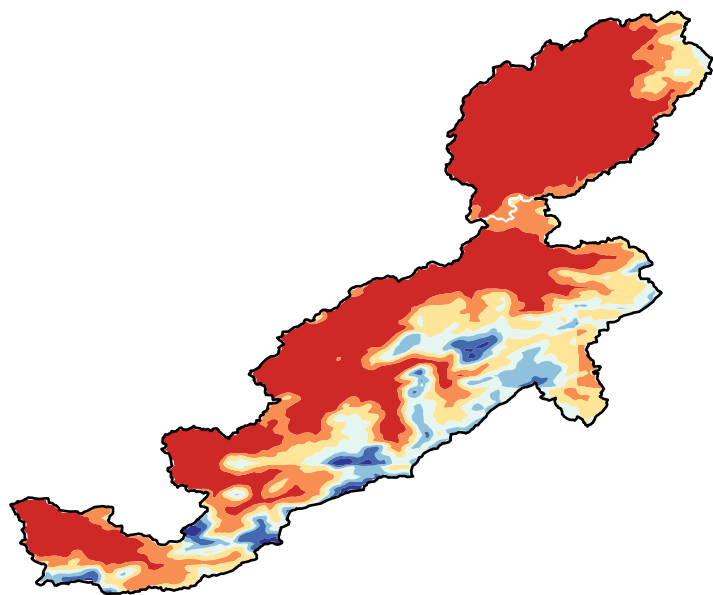
(c) (GFDL-ESM2M, 1976-2005)
