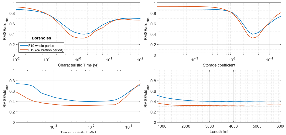
Figure S5. nRMSE criterion in function of aquifer model parameters for borehole F19 in Ploemeur. Blue curve: model calibrated over the period 1996-2012. Orange curve: model calibrated over the period 1996-2004.
