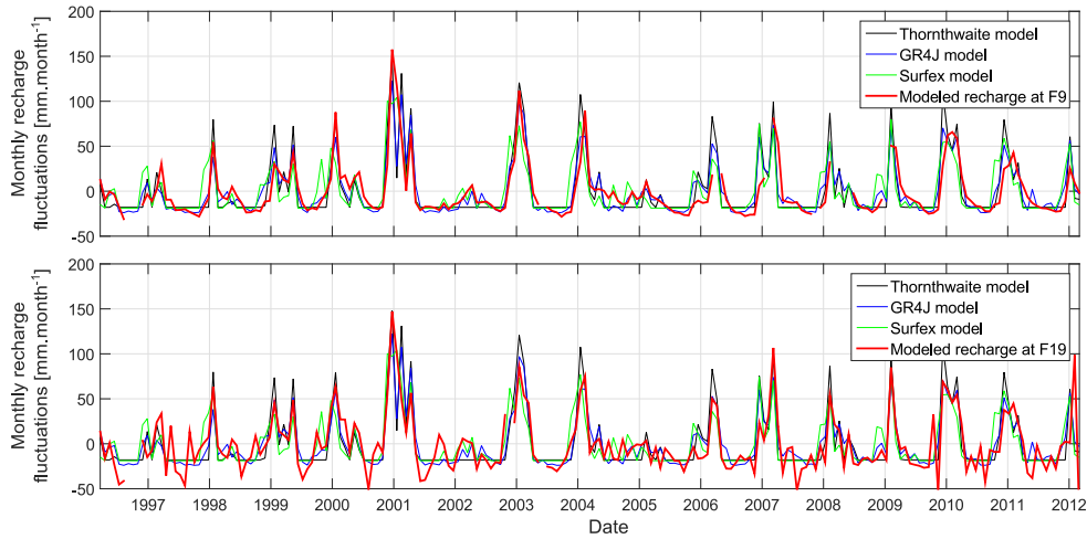
Figure S4. Comparison between recharge fluctuations (anomalies compared to the mean value) from three potential recharge models (Thornthwaite, GR4J, SURFEX) and from GW analytical model (in \text{mm}\cdot\text{month}^{-1} ) at boreholes F9 (upper graph) and F19 (lower graph) on Ploemur site.
