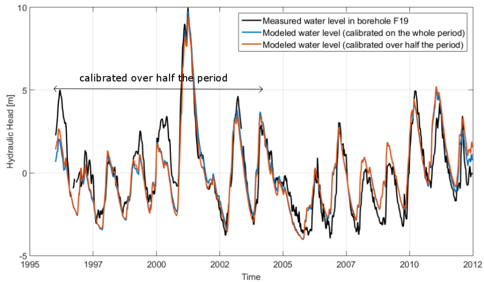
Figure S6. Comparison between observed (black line) and simulated water table fluctuations. Blue curve: model calibrated over the period 1996-2012. Orange curve: model calibrated over the period 1996-2004.
