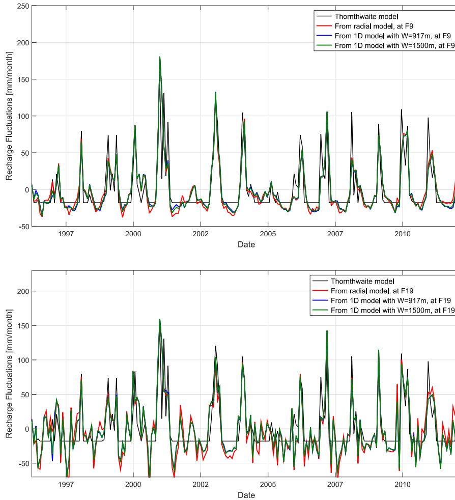
Figure S3. Comparison between potential recharge fluctuations [ \text{mm} \cdot \text{month}^{-1} ] estimated from Thornthwaite model and recharge fluctuations estimated from observed water table at boreholes F9 (upper graph) and F19 (lower graph) on Ploemur site. Recharge fluctuations from observed water table are estimated using the radial model or two 1D groundwater models with W = 917 \text{ m} and W = 1500 \text{ m} . "Fluctuations" means that time variations are expressed as anomalies compared to the mean value along the study period.
