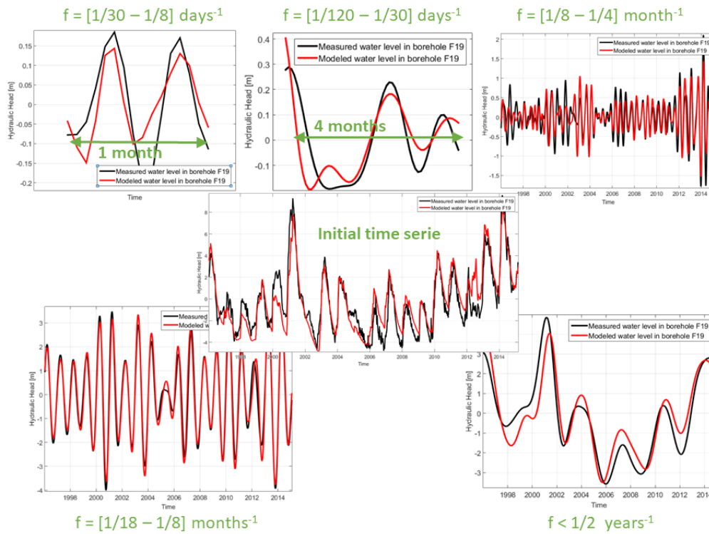
Figure S7. Water table fluctuations observed at borehole F19 (black lines). The graph in the middle represents the initial data. From initial data, five data sets of water table fluctuations are generated. For each time series, different period lengths are considered and only a range of frequencies are studied.
