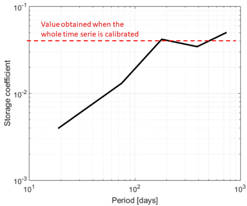
Figure S8. Estimated storage coefficient in function of the studied time scale ("Period"). Note water table fluctuations are all well reproduced by the model whatever the frequency range.
