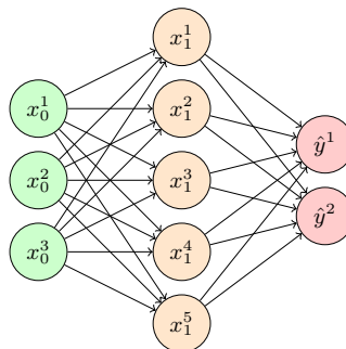
(a) Multi-layer perceptron
