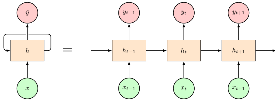
(e) Recurrent neural network
