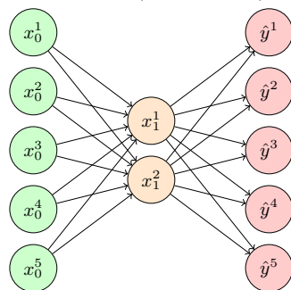
(b) Encoder-decoder
