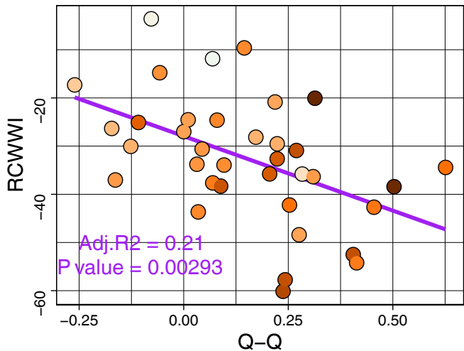
(b) Change of Mean Wintertime SPEI12 after 1980 depending on Q-QD and RC in WWI
