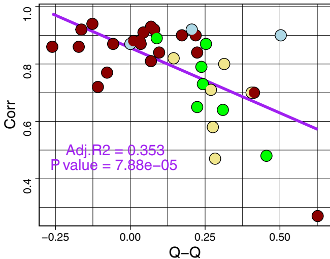
(a) Prevailing Permeability of Soils depending on Q-QD and Corr WWI/WP
