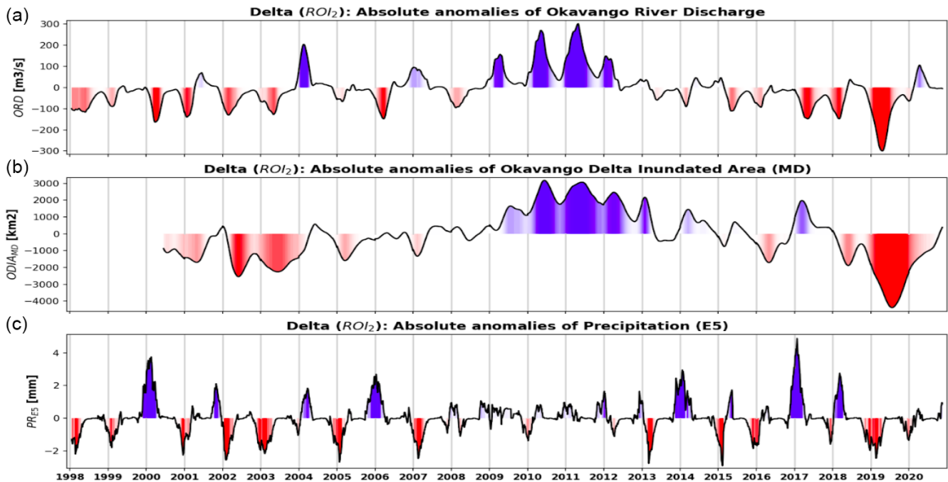
Figure 5. ORD, ODIA MD , and PR E5 time series over the Okavango delta (a–c), with the intensity of the colouring based on the z -score of the positive (blue) and negative (red) anomalies.
