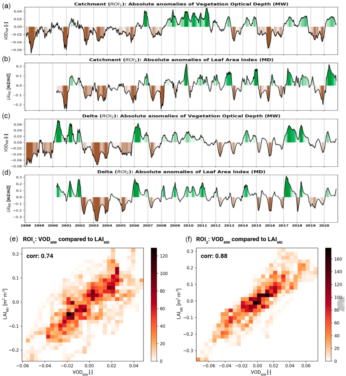
Figure 3. VOD_{MW} and LAI_{MD} anomalies over the Okavango catchment (a, b, e), with the intensity of the colouring based on the z-score of the positive (green) and negative (brown) anomalies and the Okavango delta (c, d, f) in time series and density plots. A daily time step is used from the moving average dataset.
