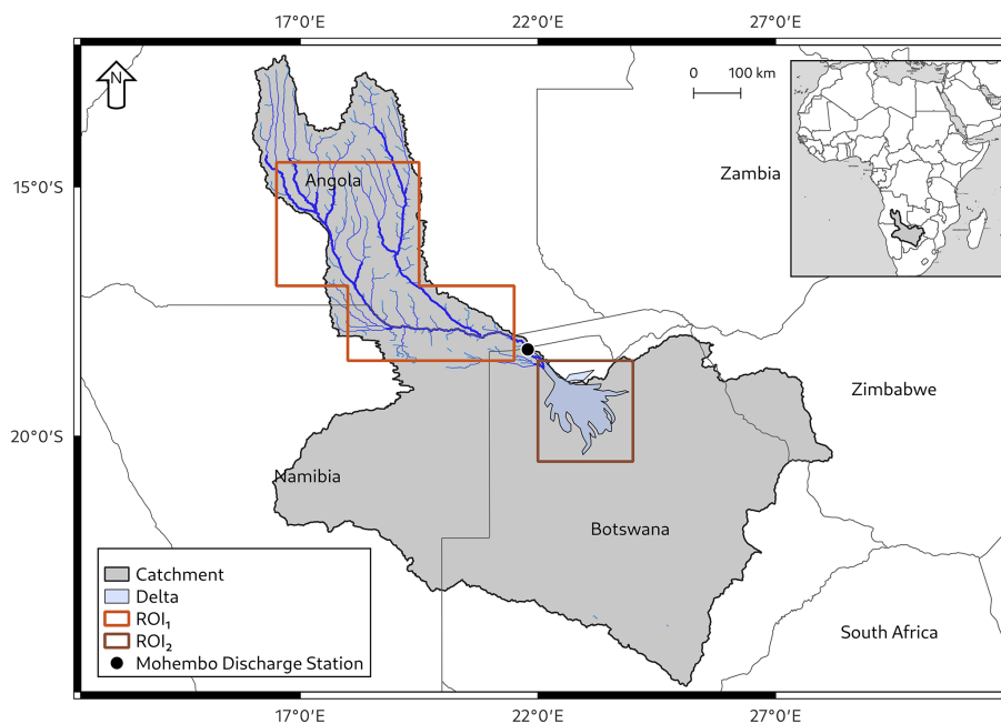
Figure 1. The research area comprising ROI 1 (a part of the upstream area of the Cubango and the Cuito rivers) and ROI 2 (the surrounding of the Okavango delta) in relation to the Okavango drainage basin (grey). The black dot marks the location of the discharge station at Mohembo.
