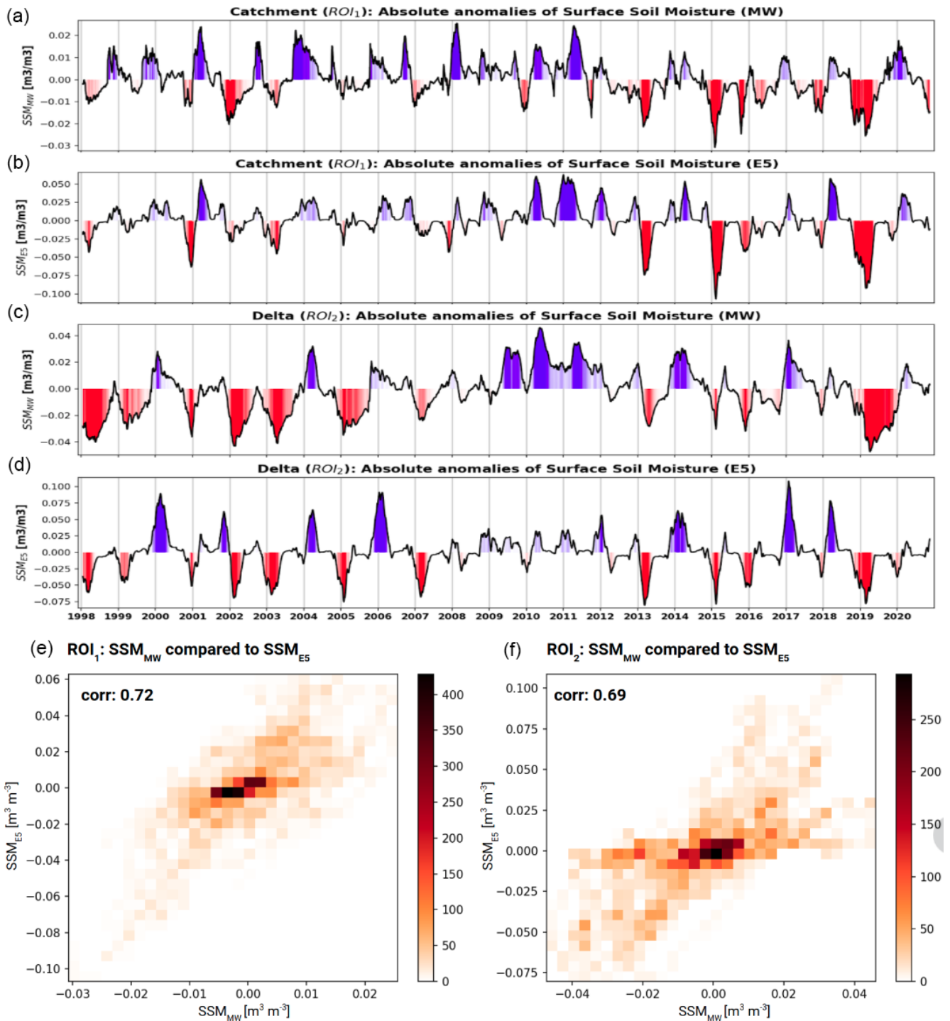
Figure 2. SSM MW and SSM E5 absolute anomalies over the Okavango catchment (a, b, e), with the intensity of the colouring based on the z-score of the positive (blue) and negative (red) anomalies and the Okavango delta (c, d, f) in time series and density plots. A daily time step is used from the moving average dataset.
