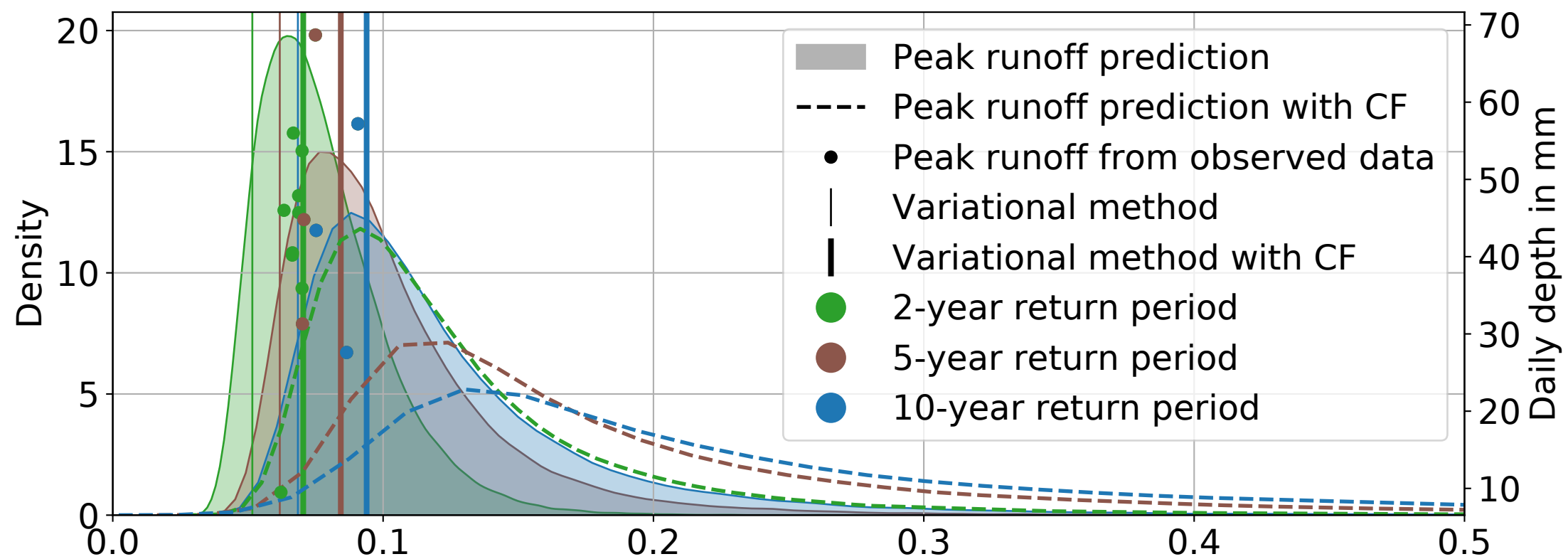
(b) D-green roof, discharge in mm/min
