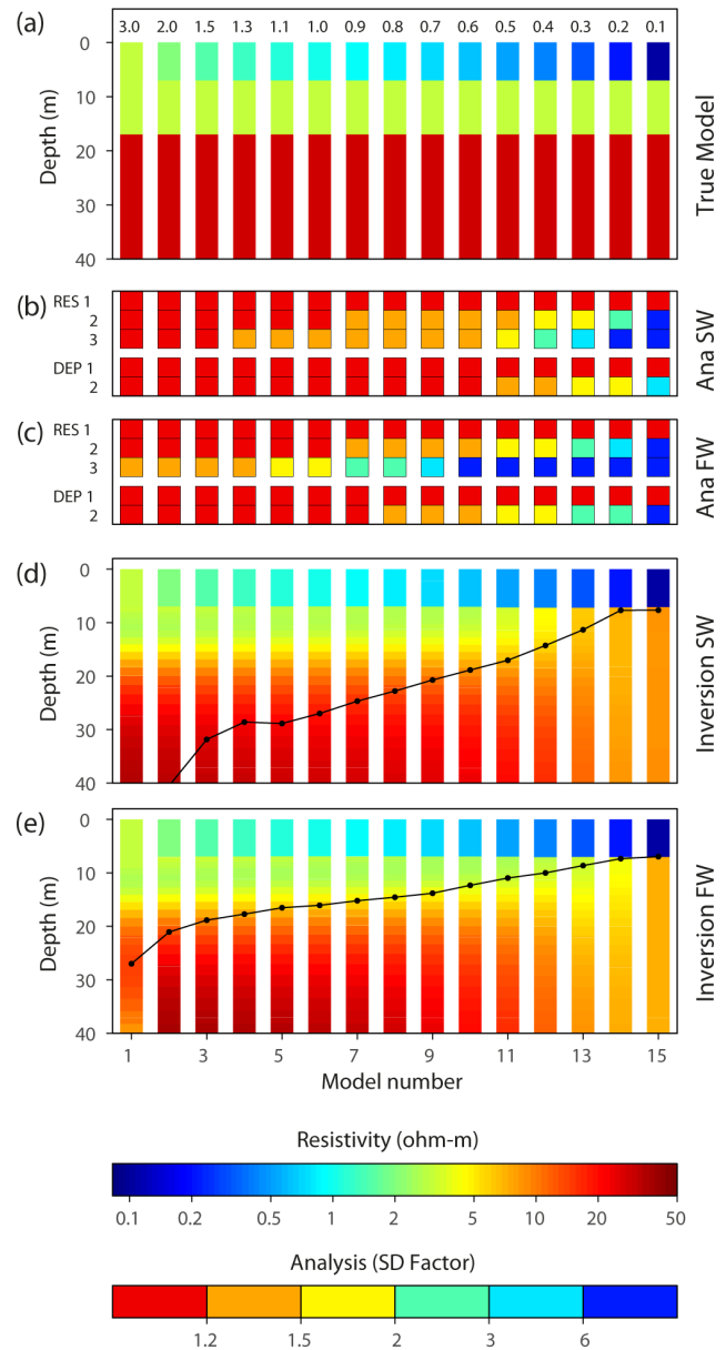
Figure 3. Model sweep 2. (a) True model. The number on top of each model bar states the resistivity of the water (resistivity of first layer). (b, c) Model parameter analysis of the true model, stated as standard deviation factor, for the SW-FloaTEM and FW-FloaTEM systems. (d, e) Inversion results for SW-FloaTEM and FW-FloaTEM systems. The black line shows the DOI.
