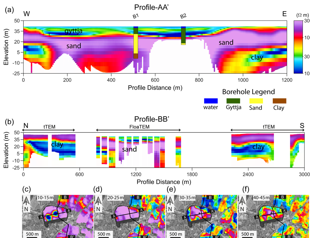
Figure 5. Results from Sunds joint tTEM and FloaTEM survey. Panels (a) and (b) show the resistivity model along profiles AA' and BB', respectively; the locations of profiles AA' and BB' are marked in Fig. 4. Note that while the elevation axis is identical, the profiles have different lengths and thereby different vertical exaggeration. Profile AA' includes lithological interpretations from available boreholes near the survey line. Note that the water column is included in the figure but only 2 m thick; panels (c)–(f) show mean resistivity maps at various depth intervals with profiles AA' and BB' indicated as solid black line. Lake Sunds is marked with a dotted black line.
