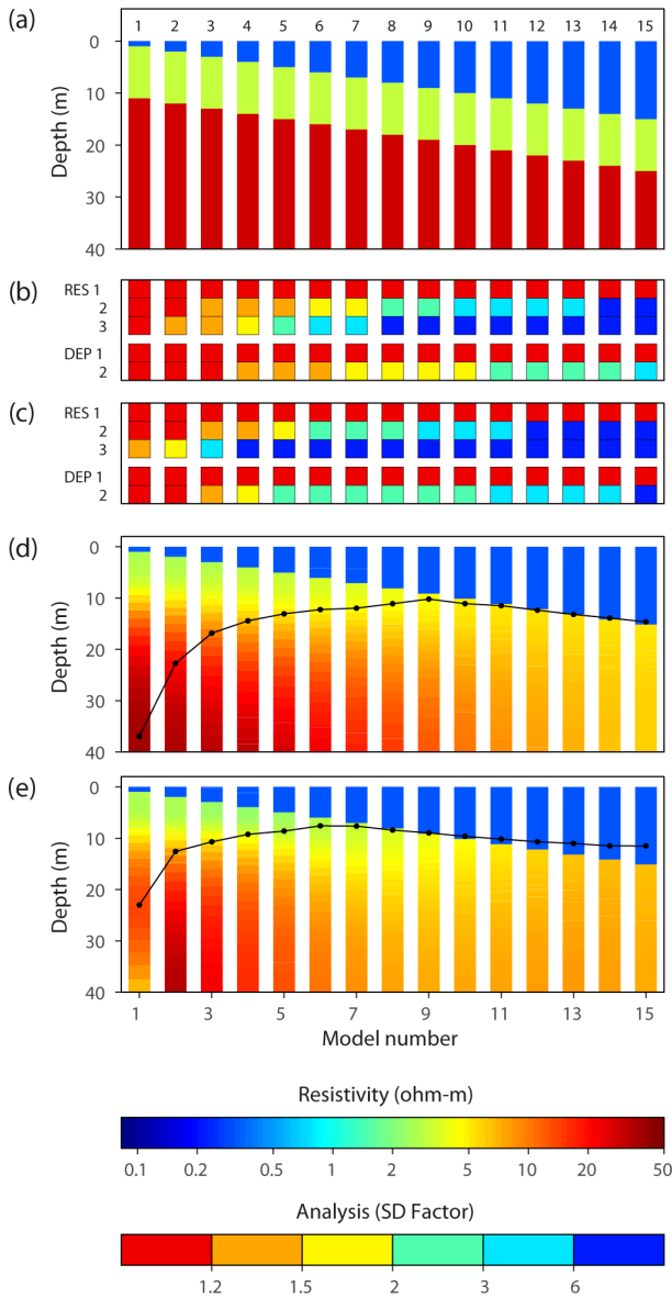
Figure 2. (a) True model. The number on top of each model bar states the water depth (thickness of first layer). (b, c) Model parameter analyses of the true models, stated as a standard deviation factor, for the SW-FloaTEM and FW-FloaTEM systems. (d, e) Inversion results for SW-FloaTEM and FW-FloaTEM systems. The black line shows the DOI.
