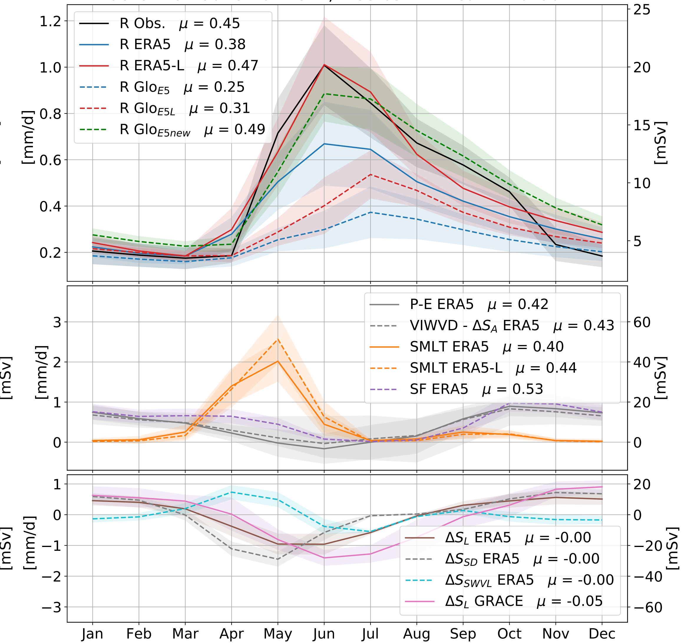
Mackenzie - Outlet: 67.45°N; -133.65°E - Area: 1726490 km 2
