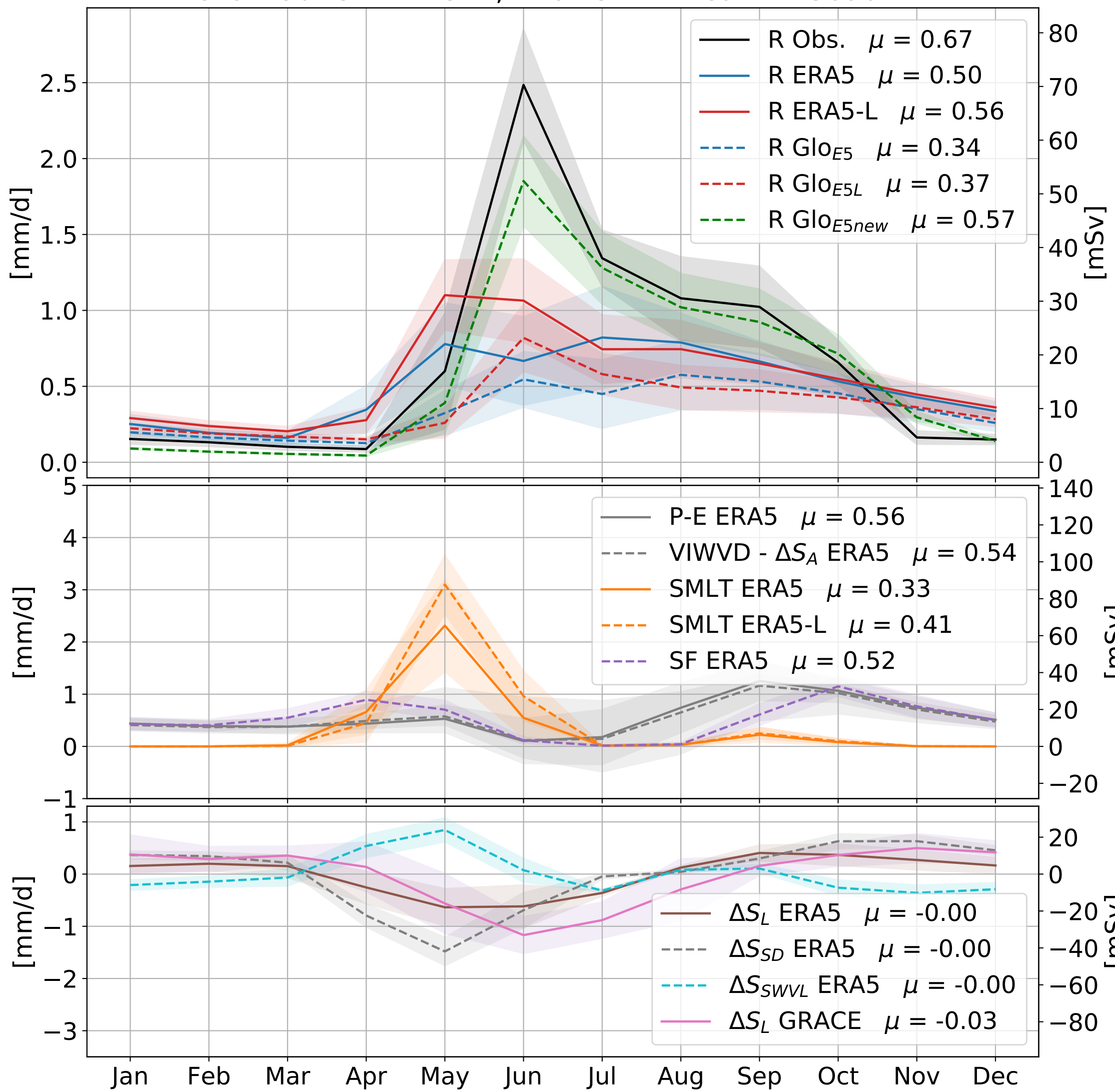
Lena - Outlet: 72.25°N; 126.75°E - Area: 2443690 km 2
