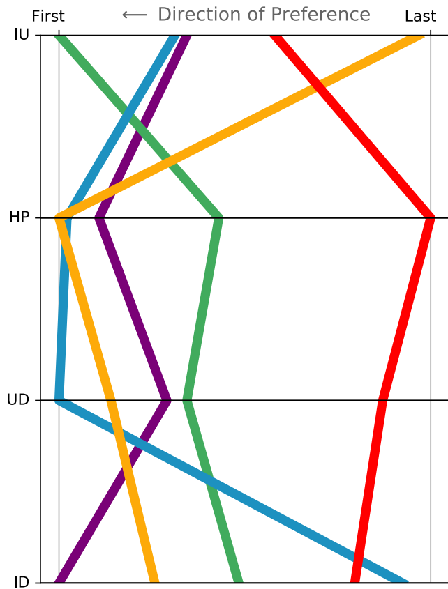
(a) minimax Robustness Ranking
