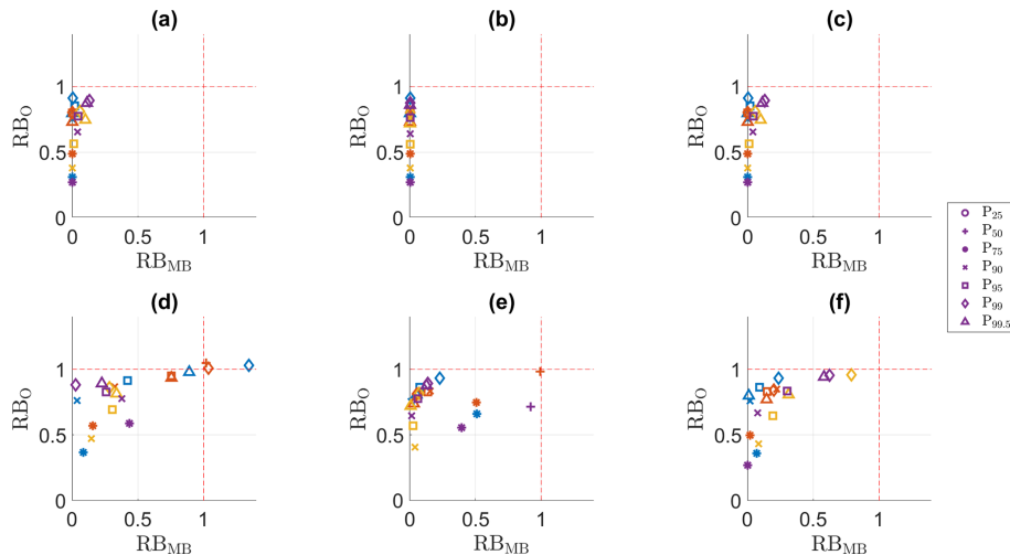
Figure 1. RB_{MB} versus RB_0 for the precipitation indices in the calibration period. (a) QDM, (b) mQDM, (c) MBCn, (d) MRQNBC, (e) dOTC, (f) R 2 D 2 . Winter: blue, spring: ochre, summer: yellow, autumn: purple.
