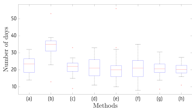
Figure 3. Box plot of the annual number of days with precipitation higher than 10 mm (ETCCDI “heavy precipitation” days; see Zhang et al., 2011) in the validation period. (a) Observations, (b) raw simulations, (c) QDM, (d) mQDM, (e) MBCn, (f) MRQNBC, (g) dOTC, (h) R^2D^2 .
