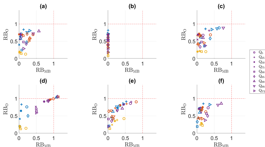
Figure 10. RB_{MB} versus RB_0 for the discharge percentiles and the 20-year return period value in the calibration period. (a) QDM, (b) mQDM, (c) MBCn, (d) MRQNBC, (e) dOTC, (f) R 2 D 2 . Winter: blue, spring: ochre, summer: yellow, autumn: purple.
