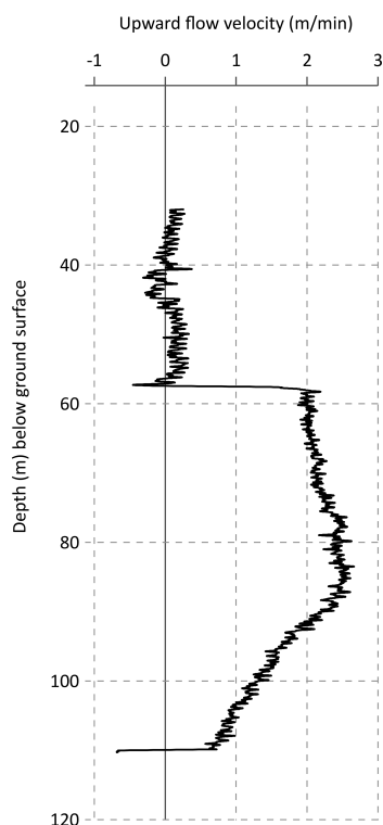
Figure 5. Example of borehole flowmeter data. The logged well is M02, while pumping is active in MP6 at a flow rate of 60 \text{ m}^3 \text{ h}^{-1} . The flow velocity measurements indicate an upward flow from approximately 110 to 55 m below the ground surface. In this same pumping experiment, downward flows are measured in other boreholes. In this case, the curve is to the left of the vertical axis (negative upward flow velocity values).
