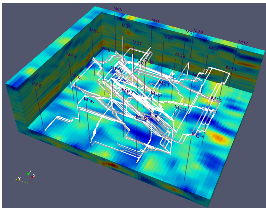
Figure 8. HES karst conduit network obtained from the combined analysis of interwell tracer tests, borehole flowmeter logs, and 3D seismic imaging data. The white and gray lines represent the main and secondary paths, respectively. The main paths are those identified via multiflow 2RNE inversion of the tracer BTCs, and the secondary paths are the additional paths identified via multiflow ADE inversion; please refer to Fig. 6.
