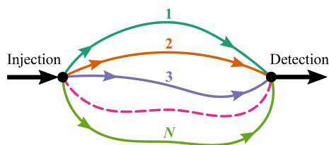
Figure 1. Schematic layout of the multiflow modeling approach implemented in MFIT software (Bodin, 2020a). The tracer transport from the injection site to the monitoring point is assumed to occur in a flow network comprising N independent one-dimensional channels.
