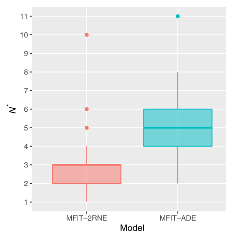
Figure 6. Minimum number N^* of flow paths between the tracer injection and pumping well pairs identified with the multiflow 2RNE model and multiflow ADE model.
