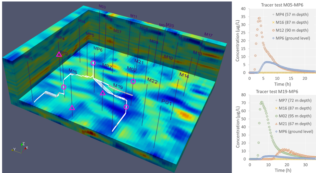
Figure 10. Verification tracer tests conducted between wells M05 (tracer injected at a 111 m depth), M19 (tracer injected at a 111 m depth), and MP6 (pumping well). The circles and triangles indicate the location of the fluorometer probes (Albillia GGUN FL22) that were or were not in the tracer path, respectively. The paths shown are those that have potentially been used by the tracer. The results obtained thus partially validate the paths M05–M12–MP6 and M19–M02–MP6. The main unknown is the connection between M19 and M21, especially as the vertical flow in M21 is downward.
