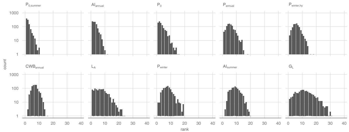
(a) c_{\text{rank winter}}
