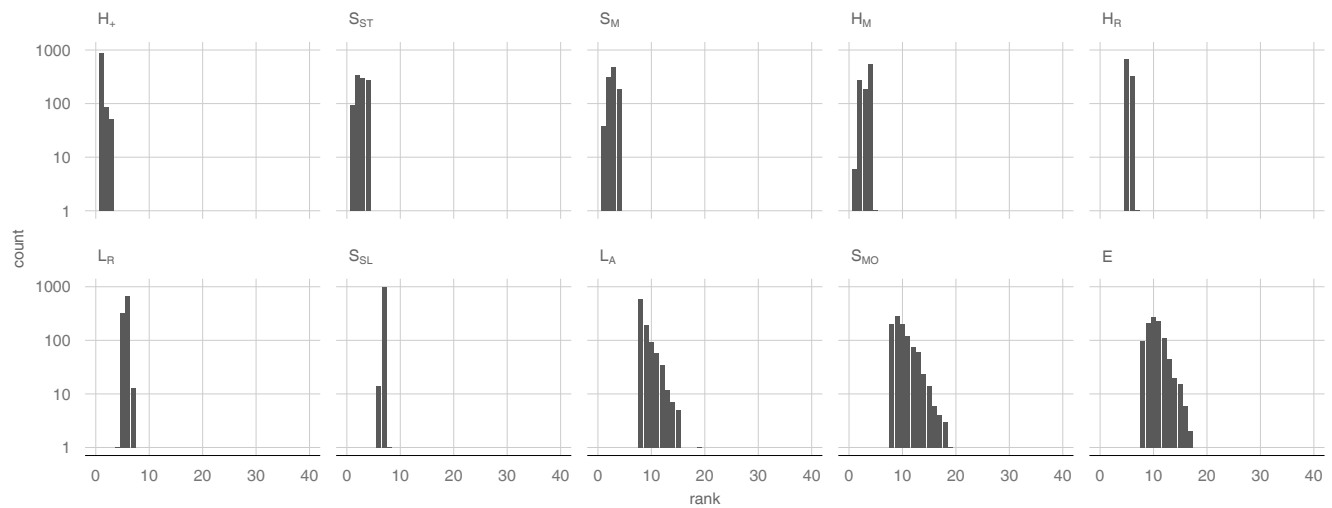
(b) c_{\text{rank summer}}
