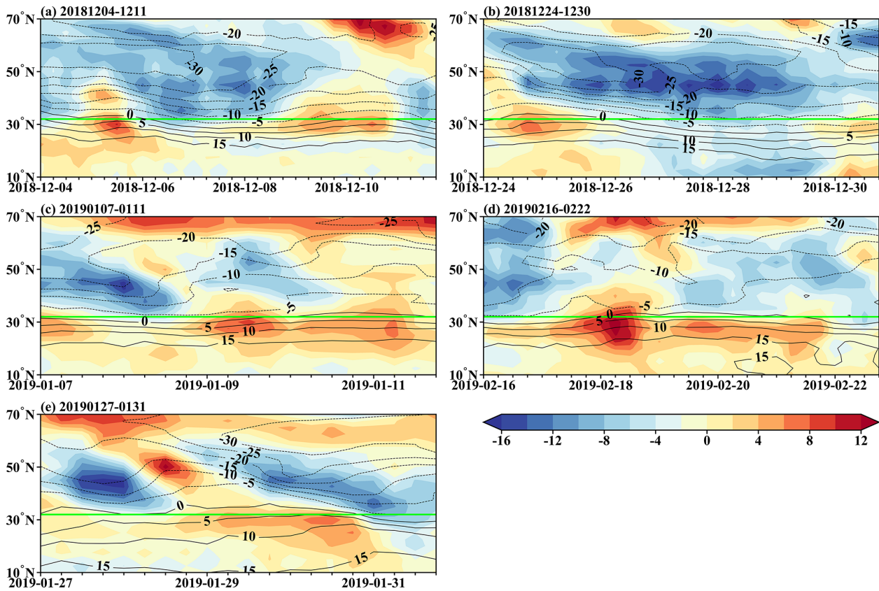
Figure 3. Latitude–time cross section of the meridional wind component (shading; units in meters per second; hereafter \text{m s}^{-1} ) and temperature (contour; units in degrees Celsius) at 850 hPa along 120^\circ \text{E} . The horizontal green lines indicate the latitude of the sampling site at Nanjing ( 32.12^\circ \text{N} ).
