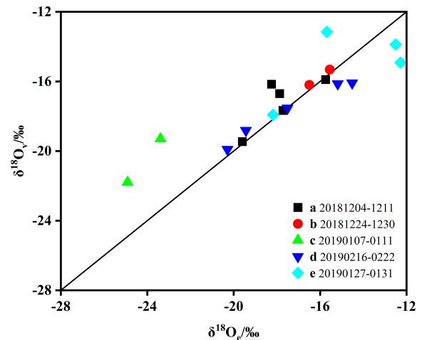
Figure 4. The relationship between observed ( \delta^{18}\text{O}_v ) and equilibrium ( \delta^{18}\text{O}_e ) vapor isotopic ratios in the five typical precipitation events. The isotopic composition of the water vapor theoretically in equilibrium with that of the precipitation ( \delta^{18}\text{O}_e ) is calculated by \delta_e = (\delta_p - \varepsilon)/\alpha , where \varepsilon is the equilibrium enrichment factor, and \alpha is the liquid-to-vapor equilibrium fractionation factor (Mercer et al., 2020). The solid black line is the line of equilibrium.
