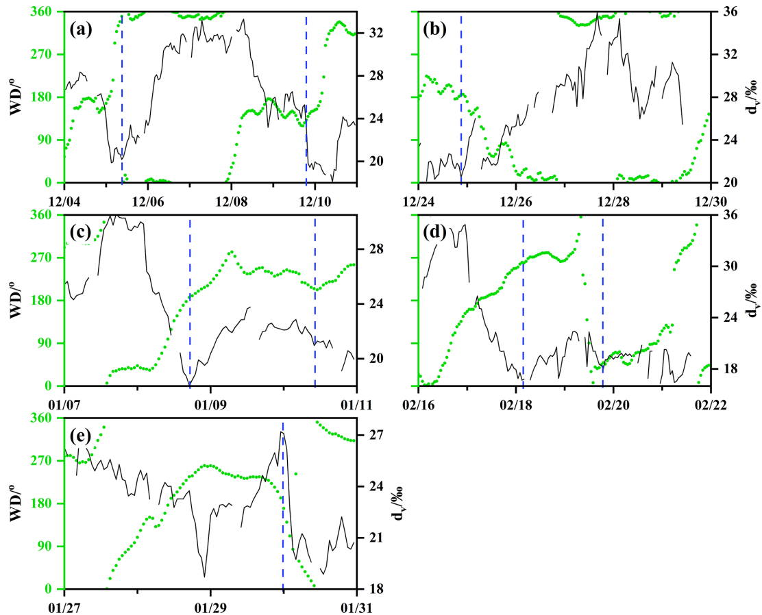
Figure 6. Time series of hourly water vapor d_v (black lines) and 850 hPa wind direction (green dots) of precipitation events. The vertical blue dashed lines indicate the different stages of precipitation events. (a) The event on 4–11 December 2018. (b) The event on 24–30 December 2018. (c) The event on 7–11 January 2019. (d) The event on 16–22 February 2019. (e) The event on 27–31 January 2019.
