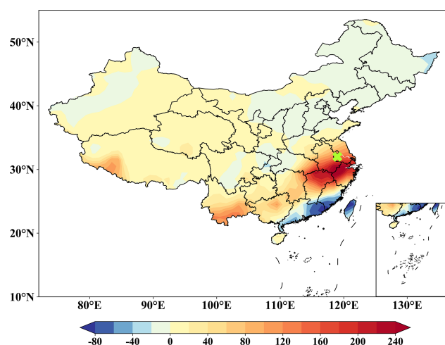
Figure 1. Winter (December–February) precipitation anomalies (shading; units in millimeters) over China in the winter of 2018–2019. The cross symbols (×) represent the sampling site at Nanjing. The anomalies were calculated with respect to the 1981–2010 climatology (precipitation data from the Global Precipitation Climatology Centre).
