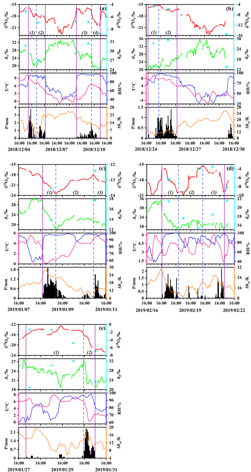
Figure 2. Time series of hourly water vapor ( \delta^{18}\text{O}_v and d_v ), daily precipitation ( \delta^{18}\text{O}_p and d_p ; cyan dots), air temperature ( T ), relative humidity (RH), precipitation amount ( P ), and atmospheric stability ( \Delta\theta_{se} ) at Nanjing. Atmospheric stability is the difference between the pseudo-equivalent potential temperature of 700 and 850 hPa ( \Delta\theta_{se} = \theta_{se700} - \theta_{se850} ). (a) The event on 4–11 December 2018. (b) The event on 24–30 December 2018. (c) The event on 7–11 January 2019. (d) The event on 16–22 February 2019. (e) The event on 27–31 January 2019. The vertical purple lines and blue dashed lines indicate the concentrated rainfall period and different stages of each precipitation event, respectively.
