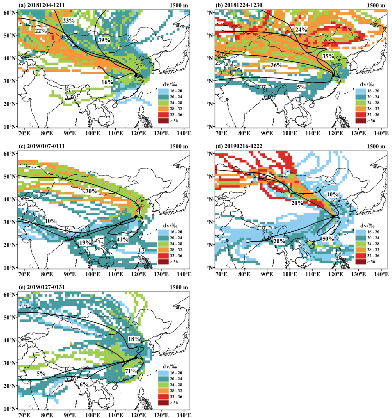
Figure 5. Concentration field of water vapor d_v for 192 h HYSPLIT back trajectories and clusters for the five typical precipitation events. The black circle indicates the location of Nanjing.
