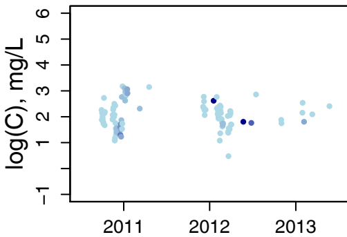
ARIDa BFI_m = 0.03 BFI_range = 0.24
