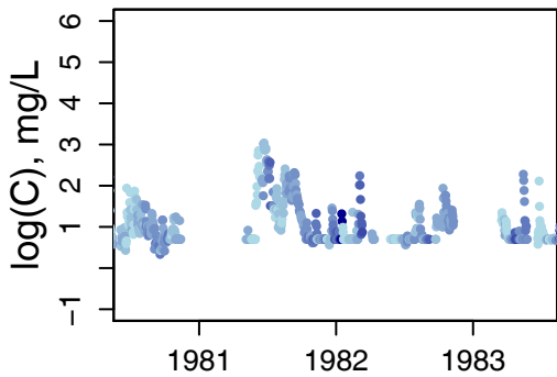
ARIDb BFI_m = 0.21 BFI_range = 0.4
