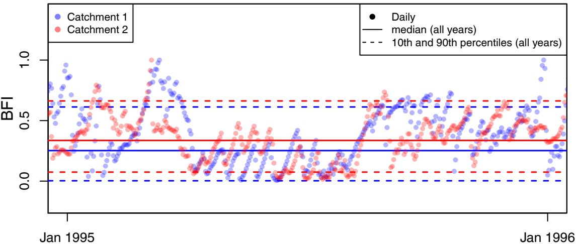
(b) Baseflow index (BFI) (1-year)
