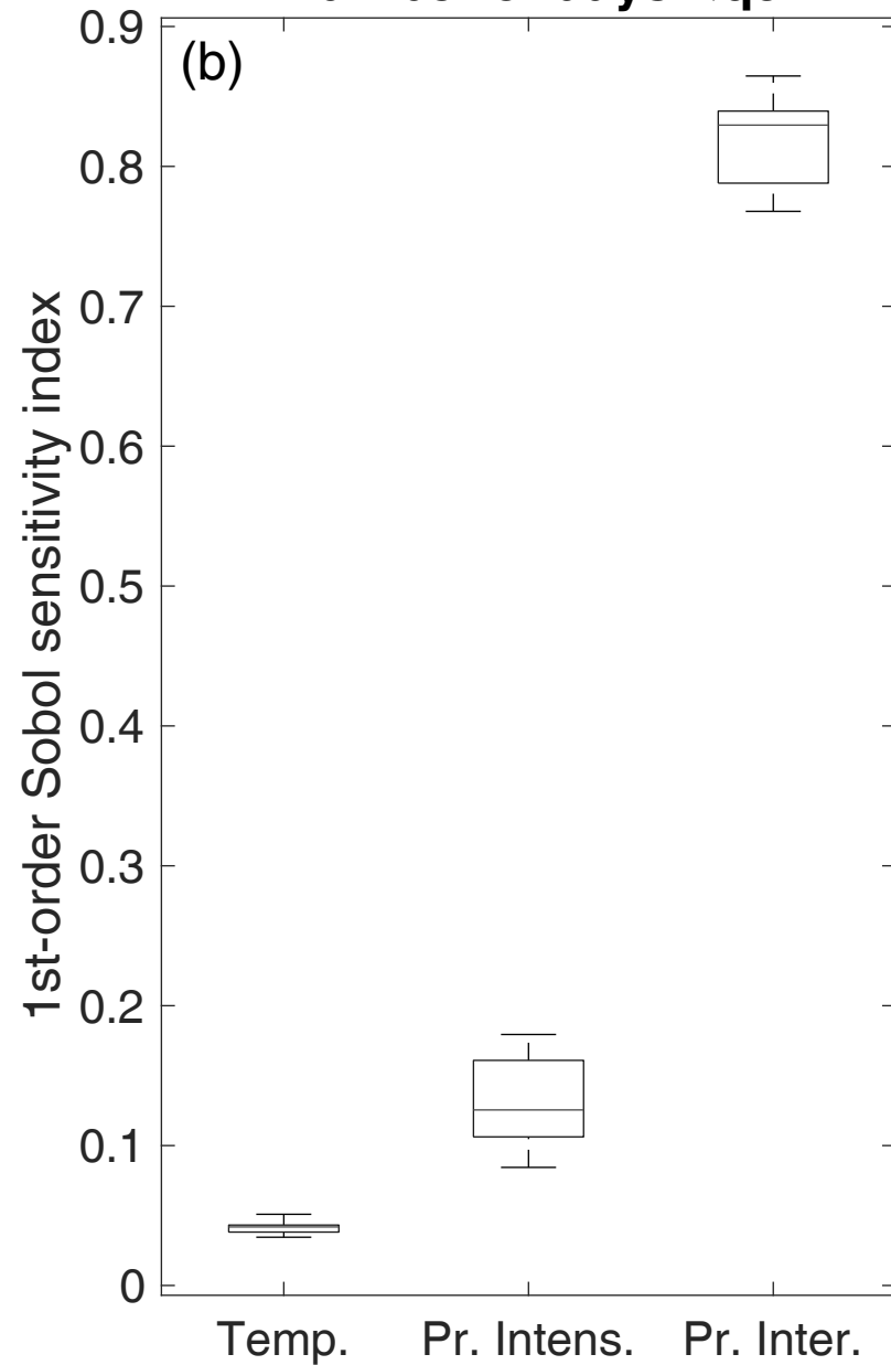
Number of days < q5
