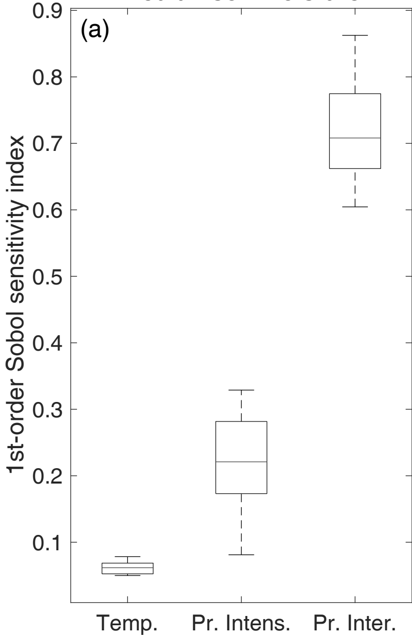
Median soil moisture
