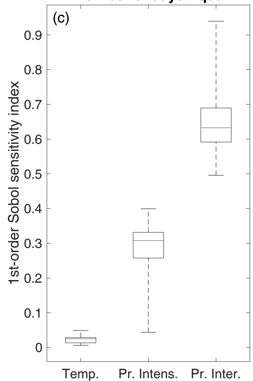
Number of days > q95
