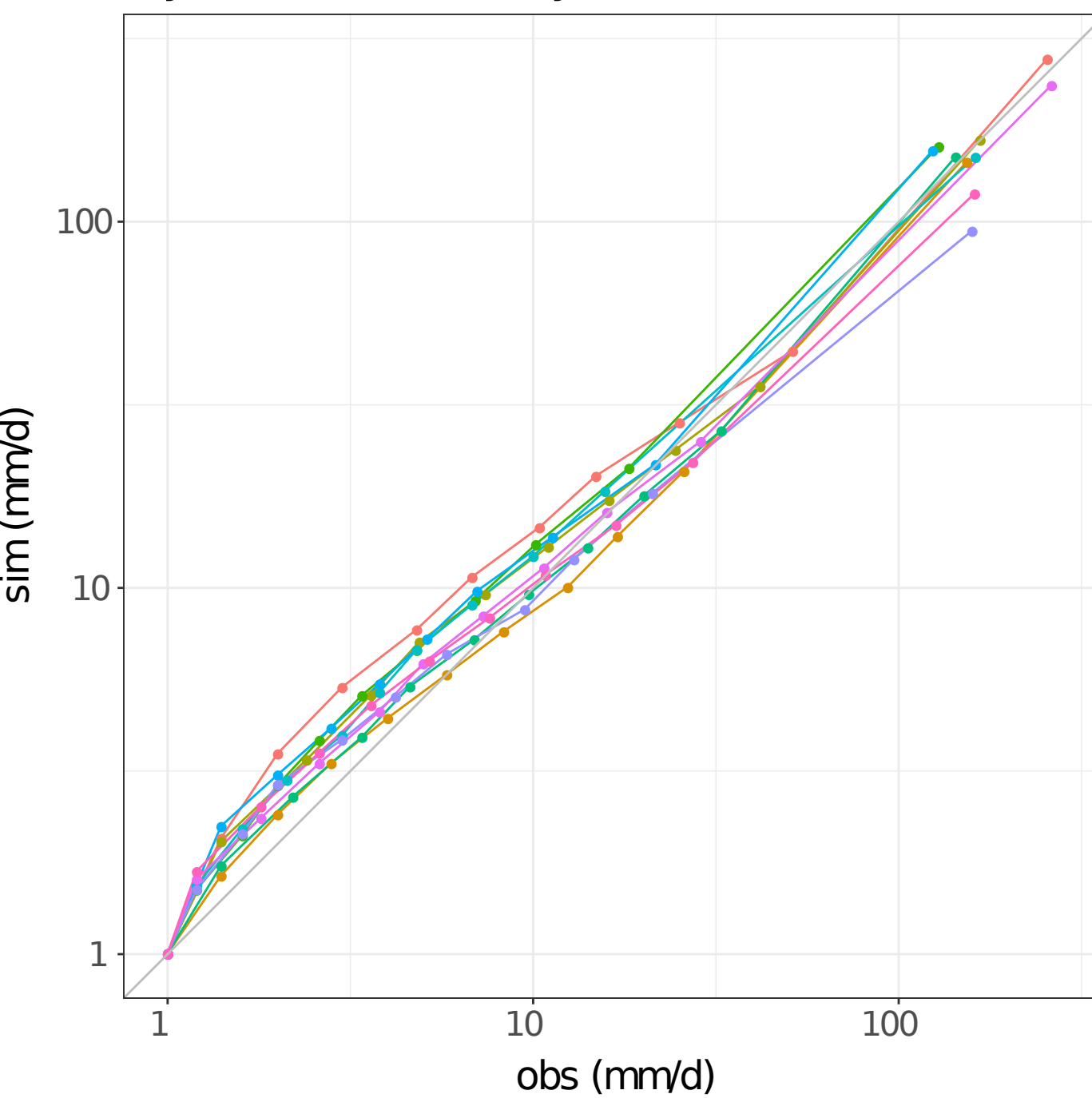
(c) Daily rainfall intensity
