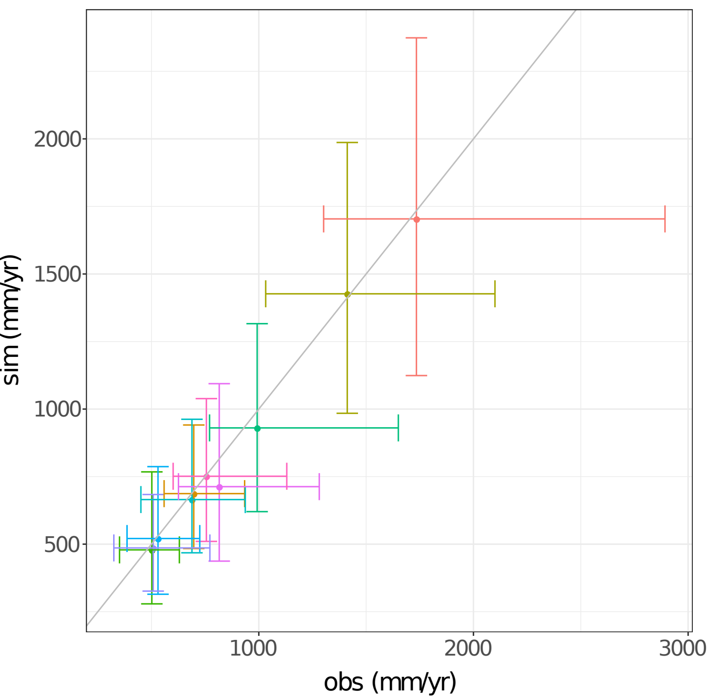
(a) Annual rainfall
