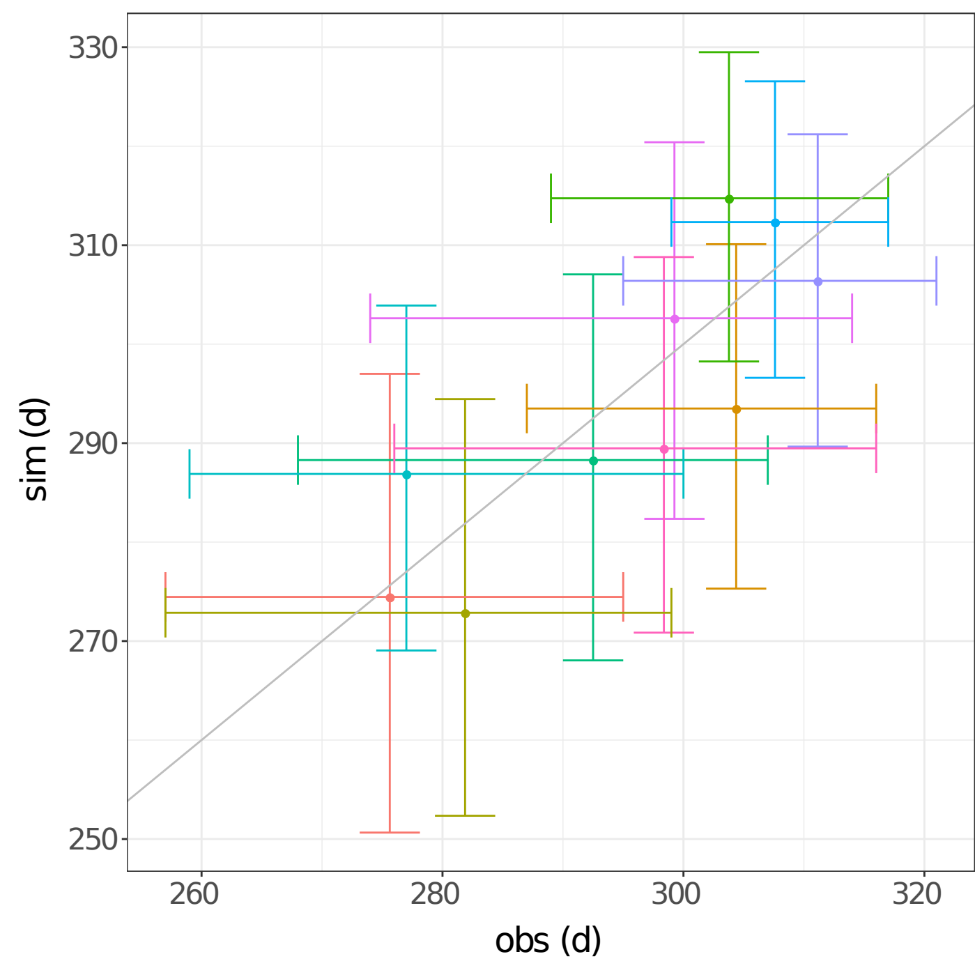
(b) Annual number of dry days
