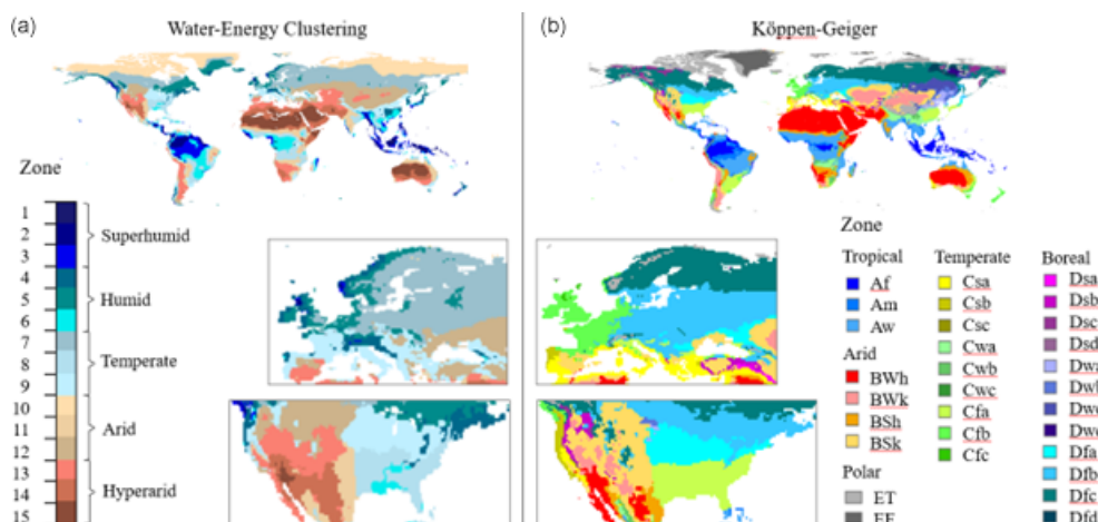
Figure 5. Spatial distribution of the Water-Energy Clustering (WEC) (a) and Köppen-Geiger (KPG) (b) classification systems. Europe and North America are magnified.
