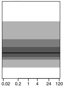
(b) annual d-GEV
