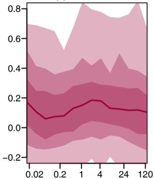
(a) annual GEV
