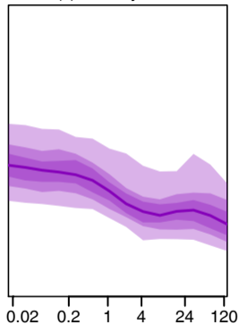
(c) monthly GEV
