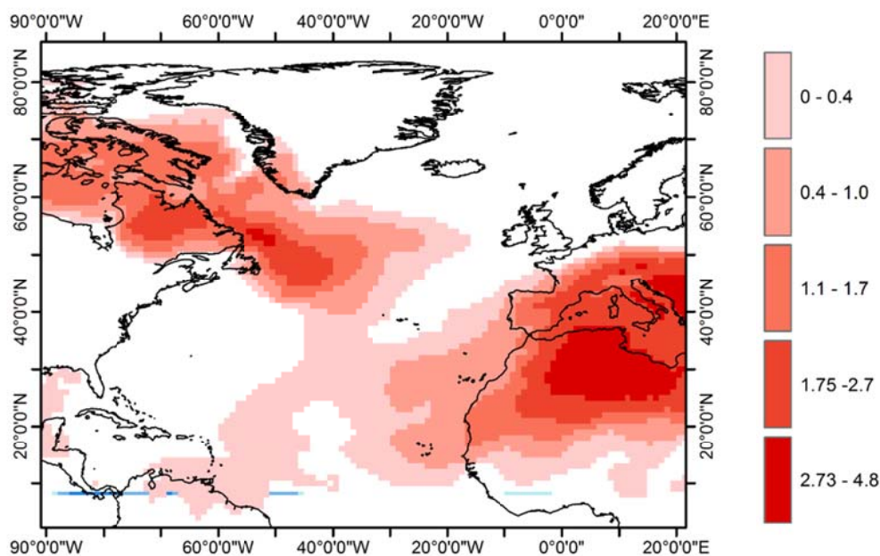
Figure S4: Temperature anomaly retrieved from 20CRV3.
