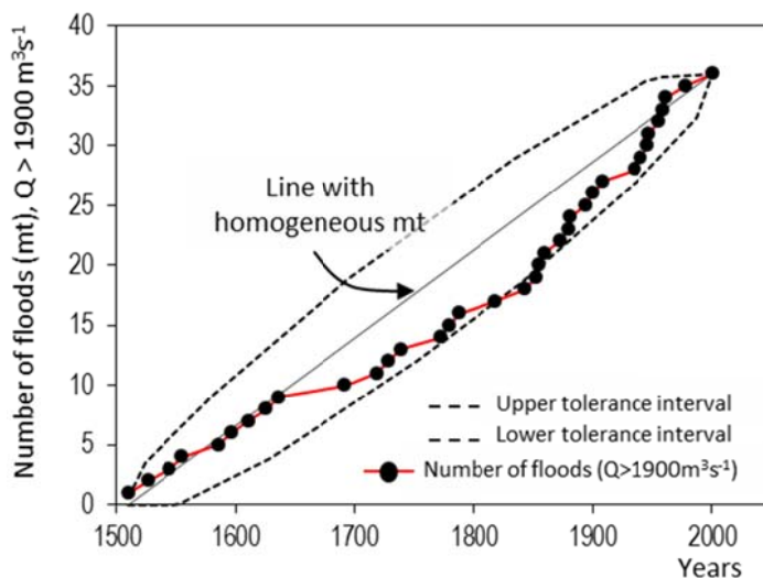
Figure S5. Stationary test on the time flood process of the Duero River over the period CE 1511–2018, for flood events equal or exceeding a discharge threshold of 1900 m 3 /s. The null hypothesis is to assume that the distribution of the number of exceedences can be described by a homogeneous Poisson process (i.e., independent and identically distributed random variables; Lang et al., 1999 and 2004). The test is passed when the accumulated flood line (red line with black dots) stays inside the 90% tolerance interval (95 and 5% quantiles; dashed lines), implying the compliance of the Poisson process hypothesis.
