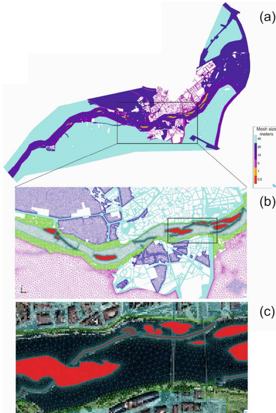
Figure S1: Numerical domain used on the two-dimensional hydraulic model (Iber) along the 13 km studied reach of the Duero River between the Carrascal gauge station and the confluence with the Valderaduey River. The elements of the mesh range from a size of 40-10 m on the floodplains, 5-1 m in the channel and 5 to 0.5 m in urban areas. a) General view of the studied reach and characteristic mesh sizes. b) Detail of the mesh size at the Zamora city area. c) Mesh size used between the Cabañas mills and the railroad bridge. Location of this area is marked by a rectangle in b. Aerial Orthophoto and LiDAR data from the Spanish National Geographic Institute, IGN; https://www.ign.es .
