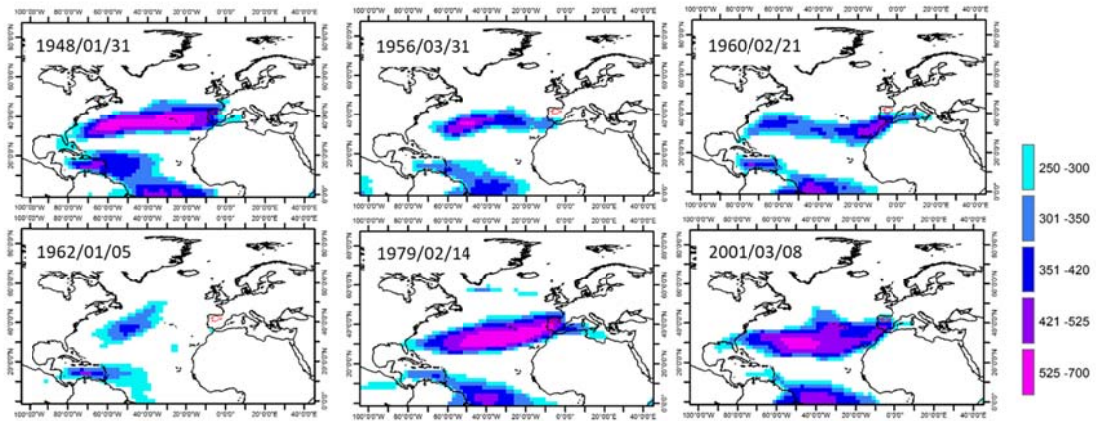
Integrated vapor transported ( \text{kg m}^{-1} \text{s}^{-1} ) - composite flood day (-10:1)
