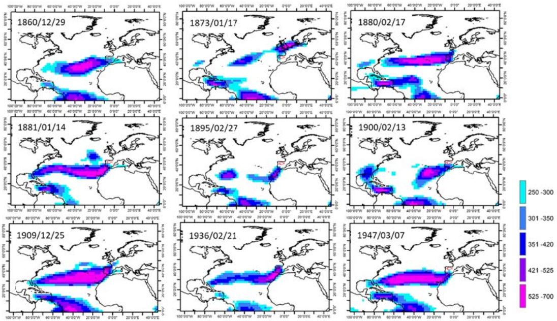
Integrated vapor transported ( \text{kg m}^{-1} \text{s}^{-1} ) - composite flood day (-10:1)
