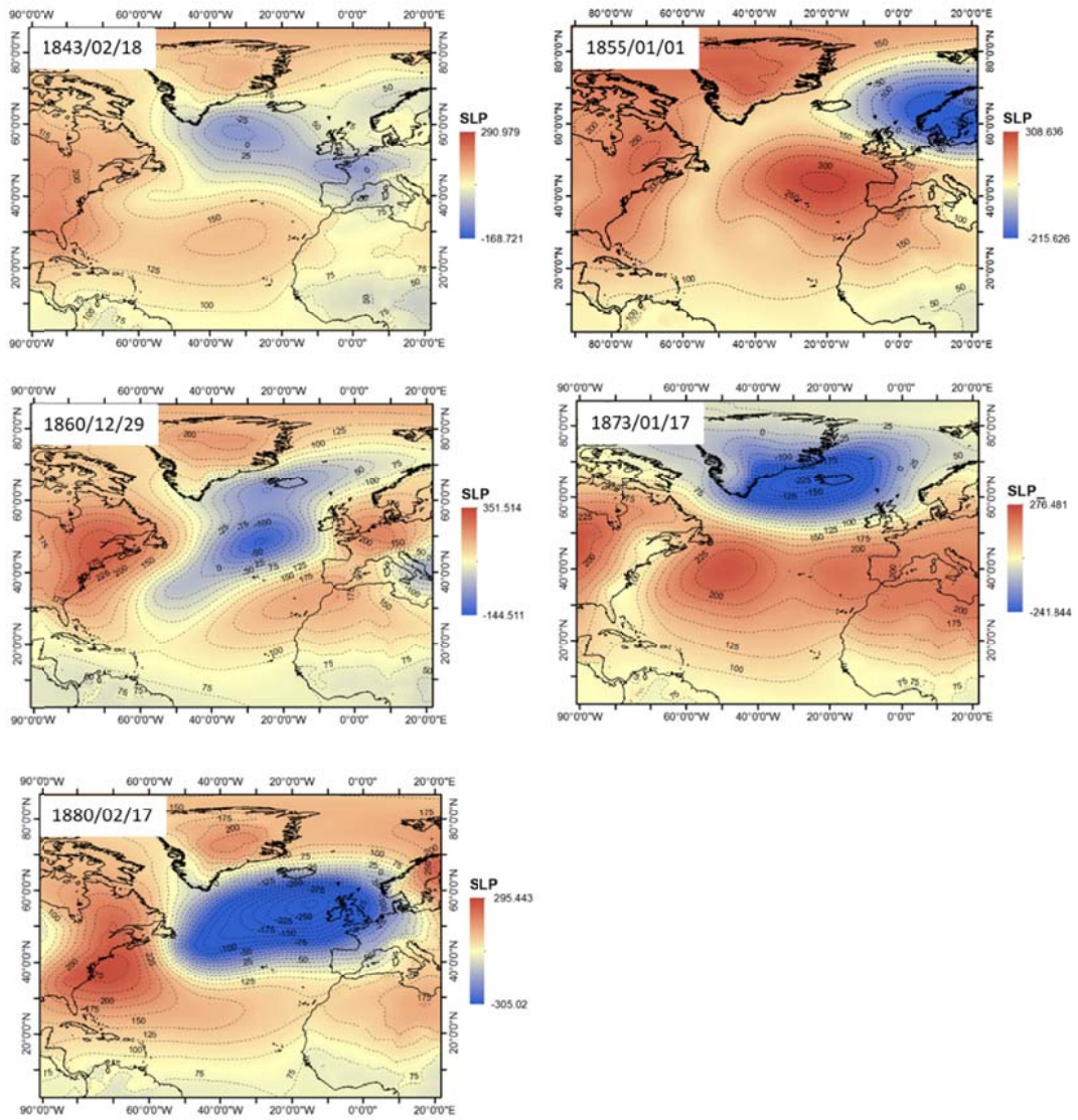
Figure S2: Chart displaying the composite (-5 days) SLP related to each flood previous 1881.
