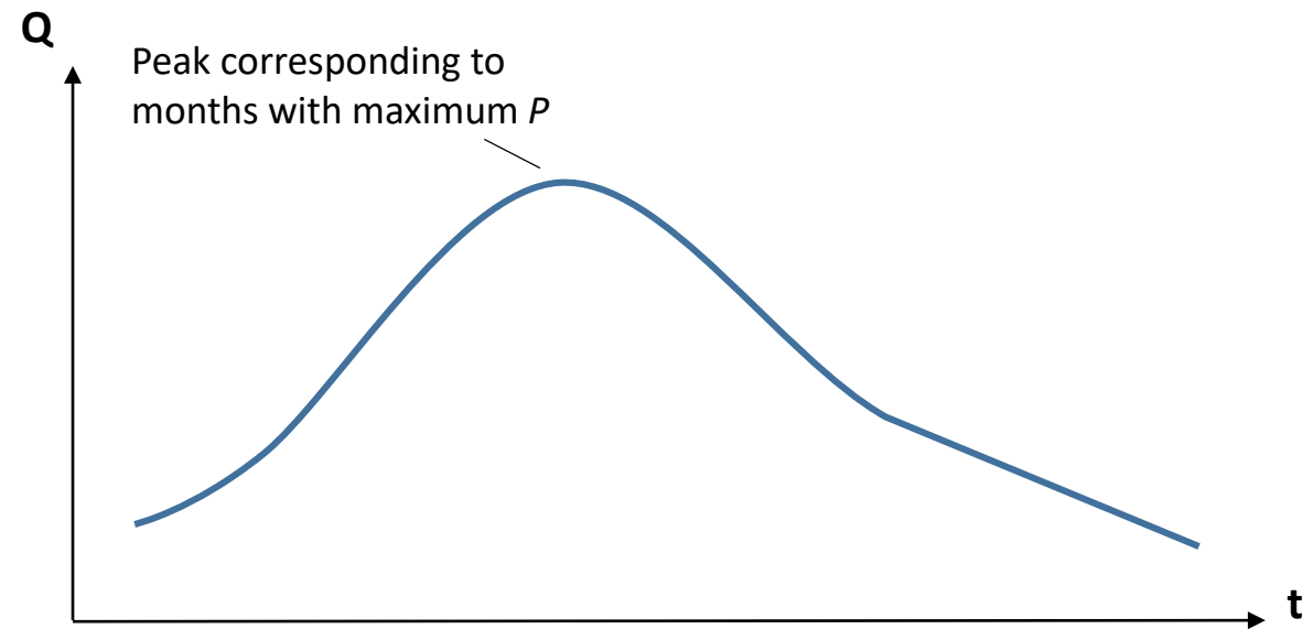
Rain-dominated
