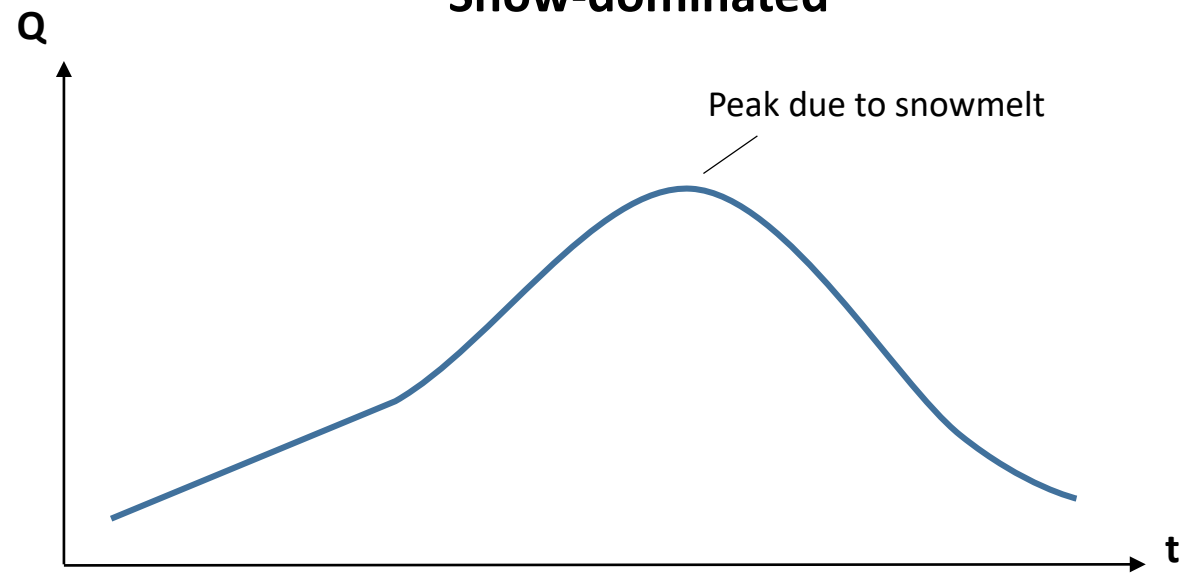
Snow-dominated
