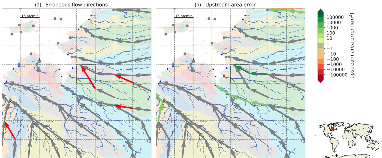
Figure C3. Largest basin (914 km 2 ) with a relative upstream area error of more than 10% at the 30 arcsec resolution indicated with a highlighted cell. See the caption of Fig. C1 for a full description.
