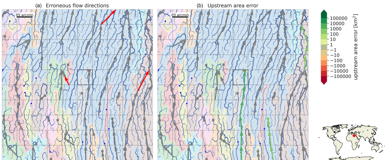
Figure C4. Largest basin (16717 km 2 ) with a relative upstream area error of more than 10% at the 5 arcmin resolution indicated with a highlighted cell. See the caption of Fig. C1 for a full description.
