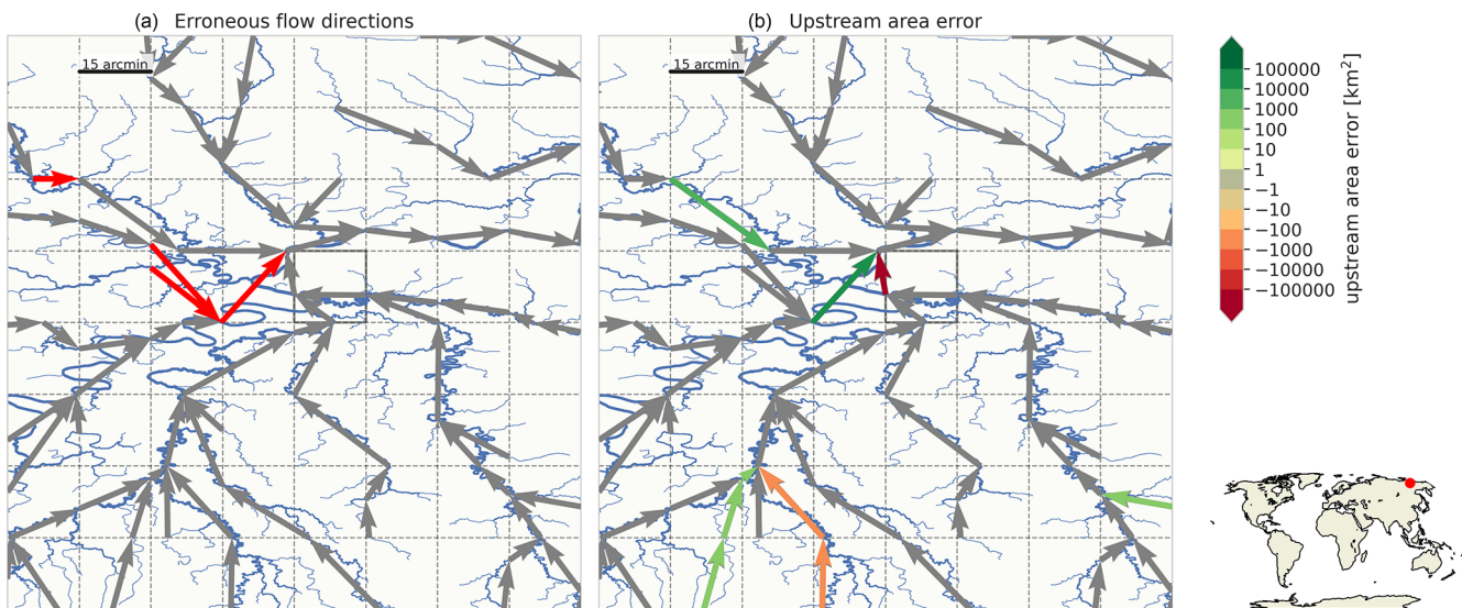
Figure C6. Second-largest local upstream area error ( -220\,876\text{ km}^2 ) at the 15 arcmin resolution indicated with a highlighted cell. See the caption of Fig. C1 for a full description.
