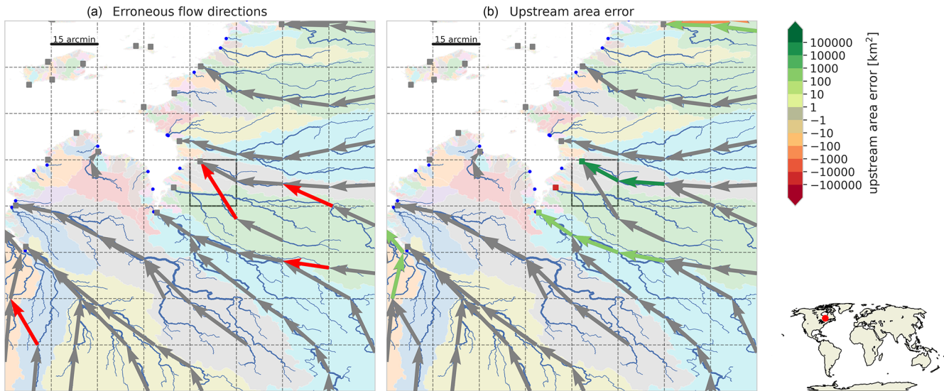
Figure C5. Largest basin ( 42\,017\text{ km}^2 ) with a relative upstream area error of more than 10% at the 15 arcmin resolution indicated with a highlighted cell. See the caption of Fig. C1 for a full description.
