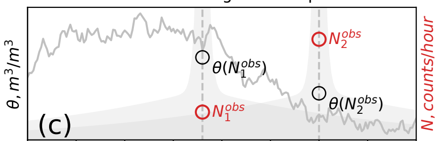
From N^{obs} to avg. \theta in footprint
