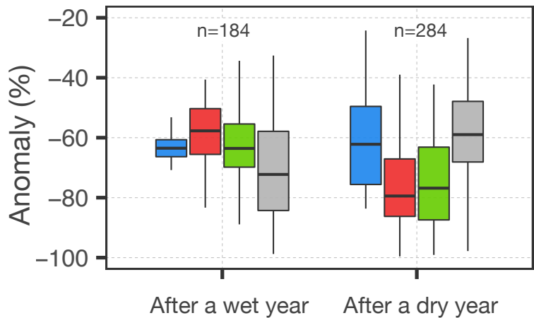
(a) Extreme & severe droughts Snow-dominated catchments
