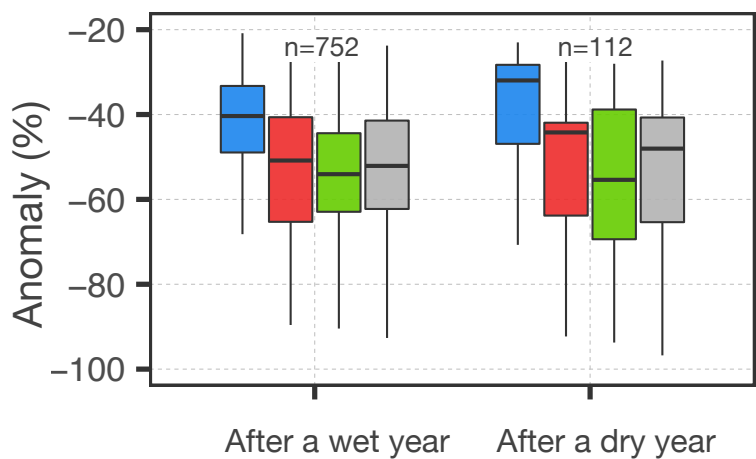
(c) Extreme & severe droughts Pluvial catchments
