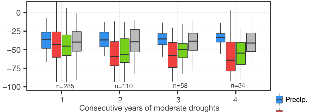
(b) Moderate & mild droughts Snow-dominated catchments
