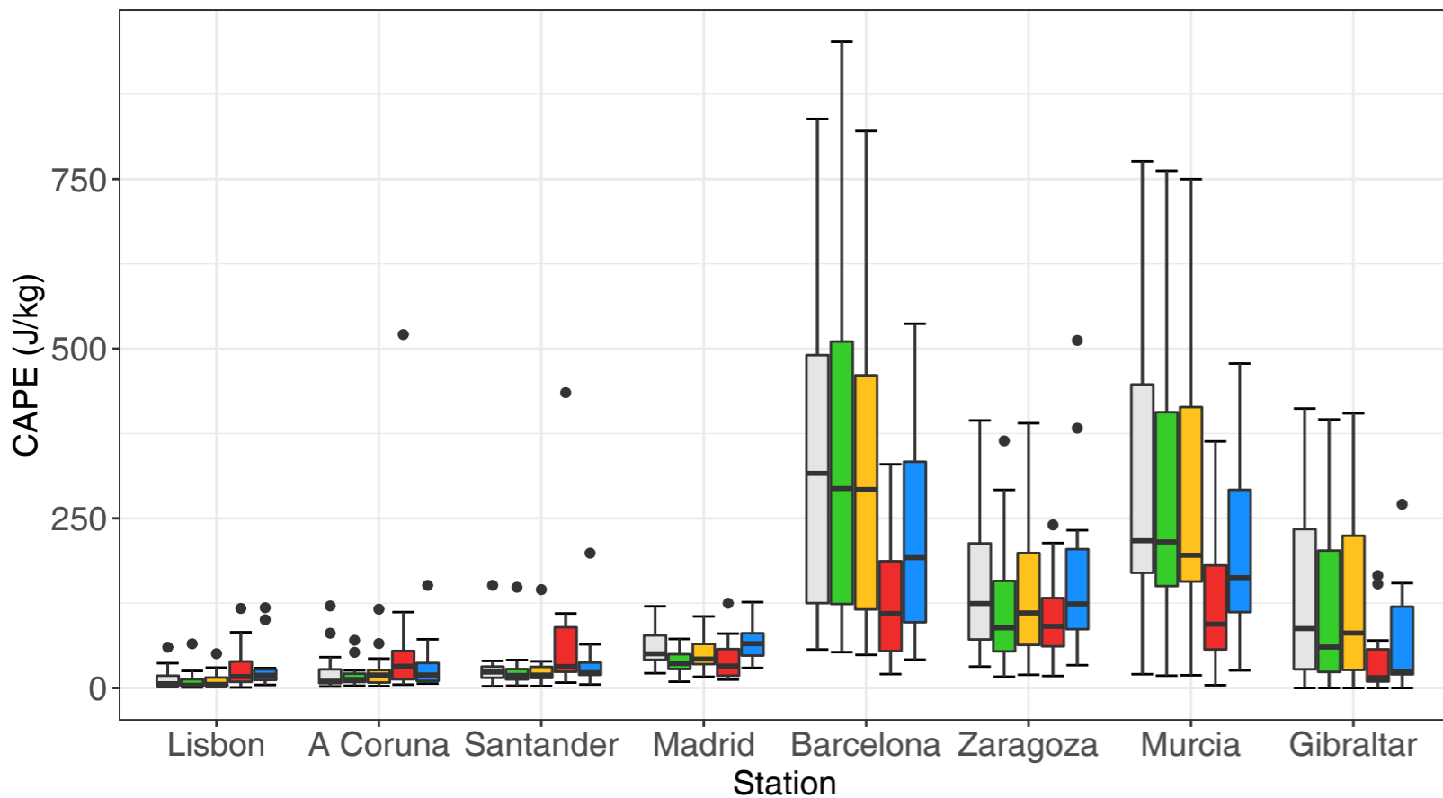
(c) CAPE – Summer JJA (Monthly data)
