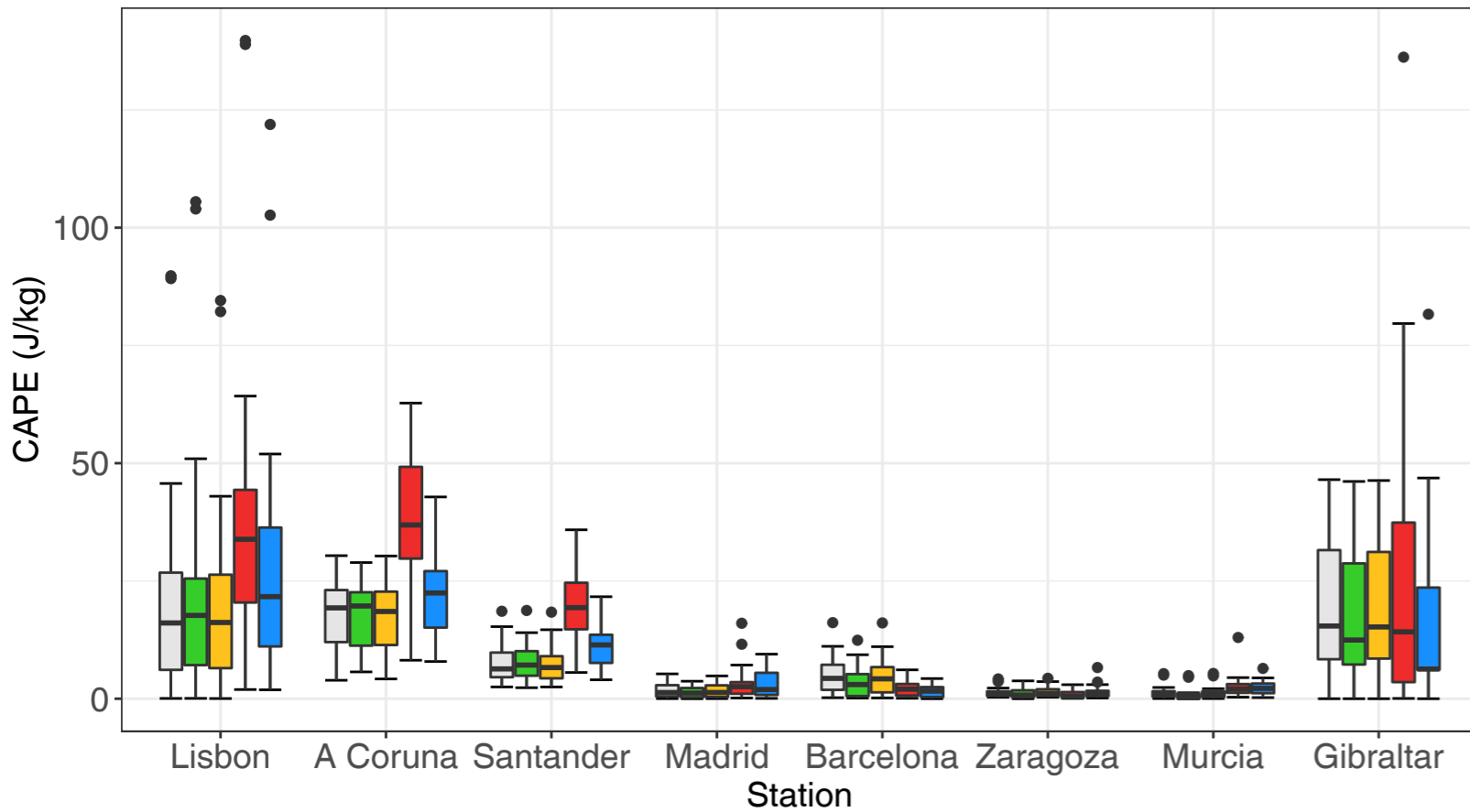
(a) CAPE – Winter DJF (Monthly data)
