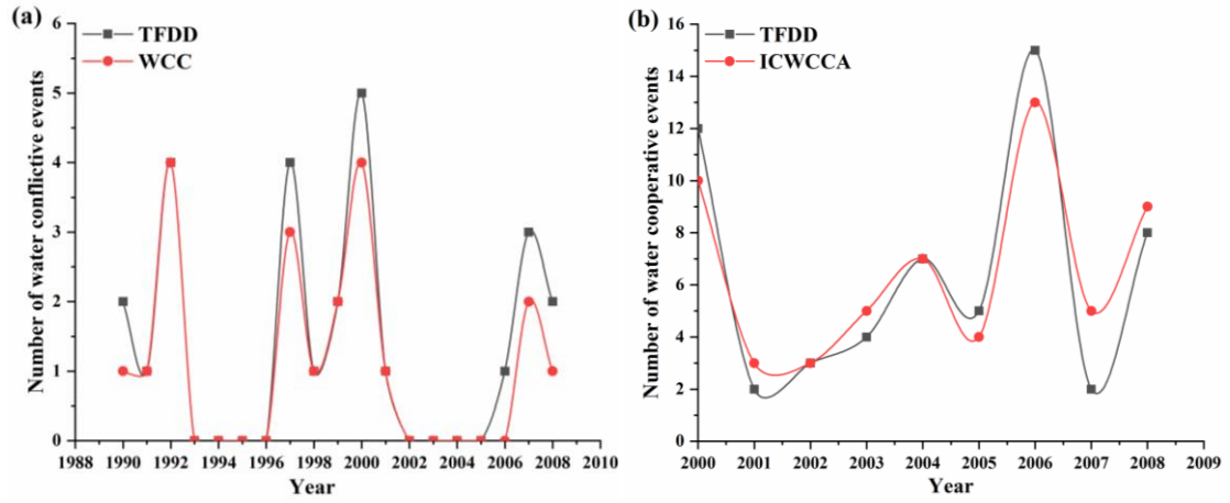
Figure S1: Comparison of the number of water conflictive events in the TFDD and WCC datasets (a) and the number of water cooperative events in the TFDD and ICWCCA datasets (b).
