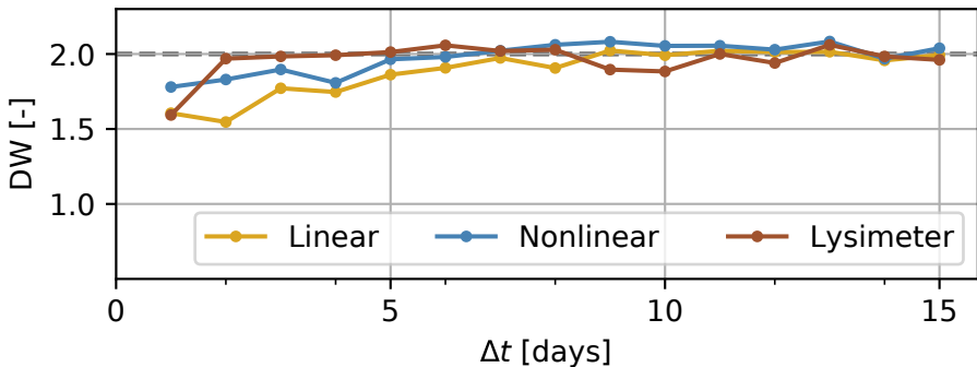
ARMA(1,1) Noise model
