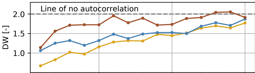
AR(1) Noise model
