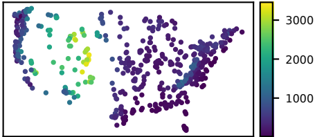
(b) Basin Elevation [m]
