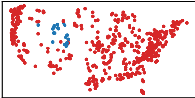
(a) Anomalous NLDAS Basins
