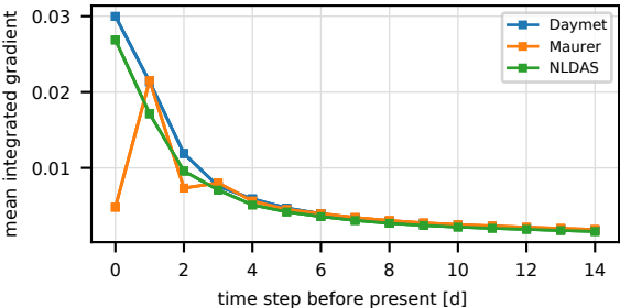
Mean Integrated Gradient over different time lags
