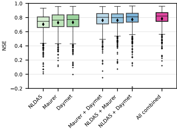
LSTM performance using different forcing inputs
