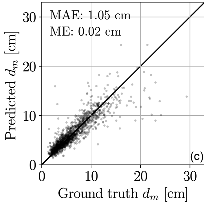
GRAINet d_m
