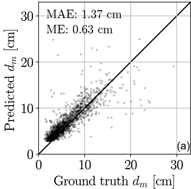
GRAINet frequency
