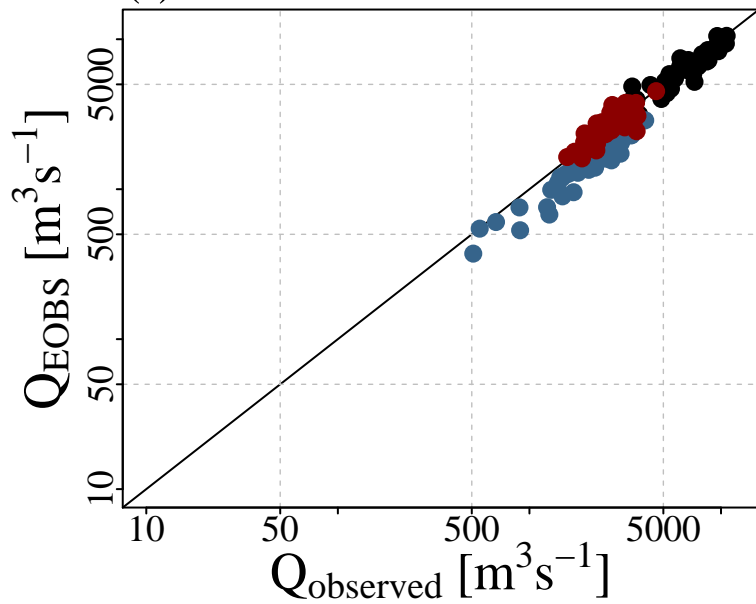
(f) MAX Observed vs. EOBS
