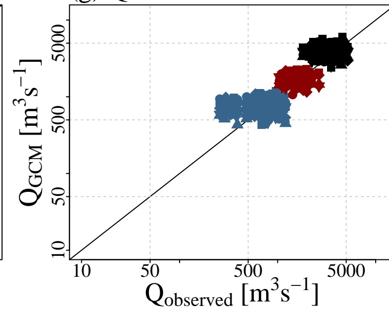
(g) Q90 Observed vs. GCMs
