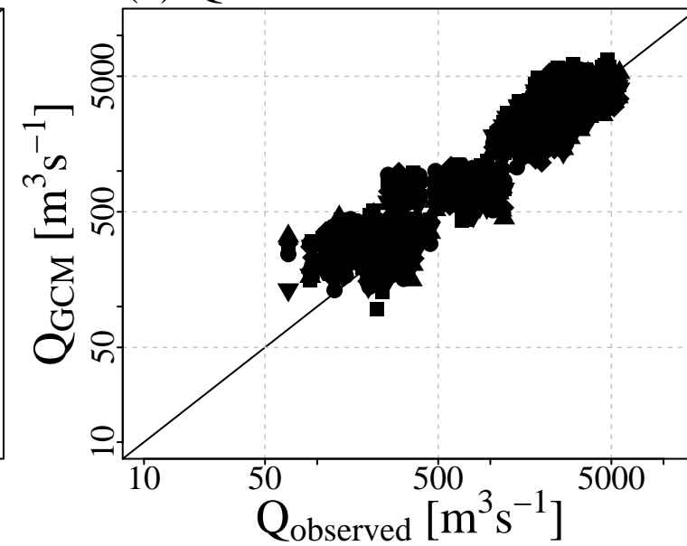
(c) Q90 Observed vs. GCMs
