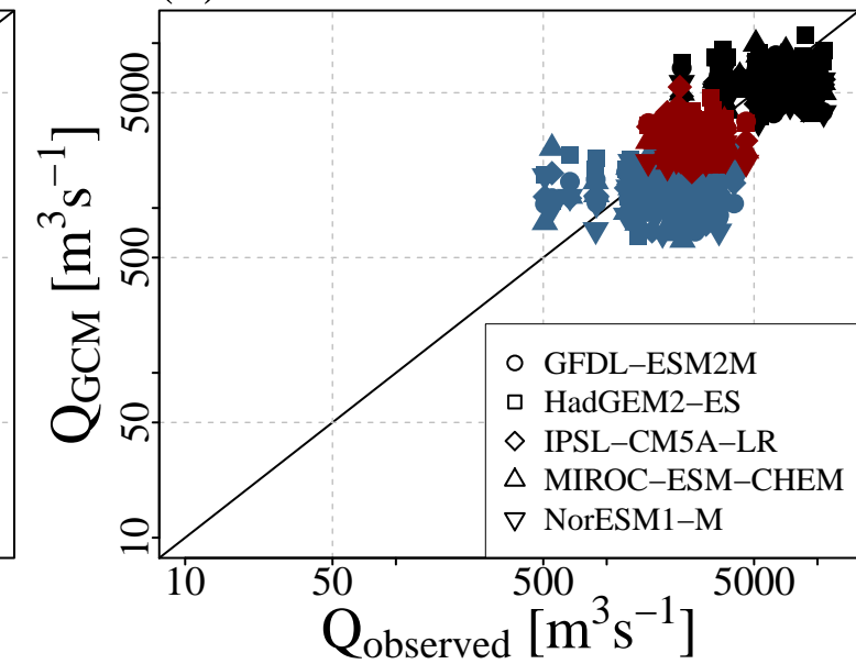
(h) MAX Observed vs. GCMs
