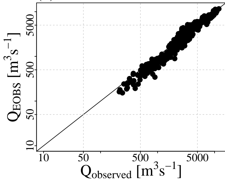
(b) MAX Observed vs. EOBS
