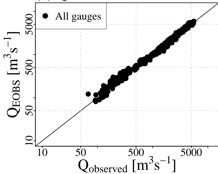
(a) Q90 Observed vs. EOBS
