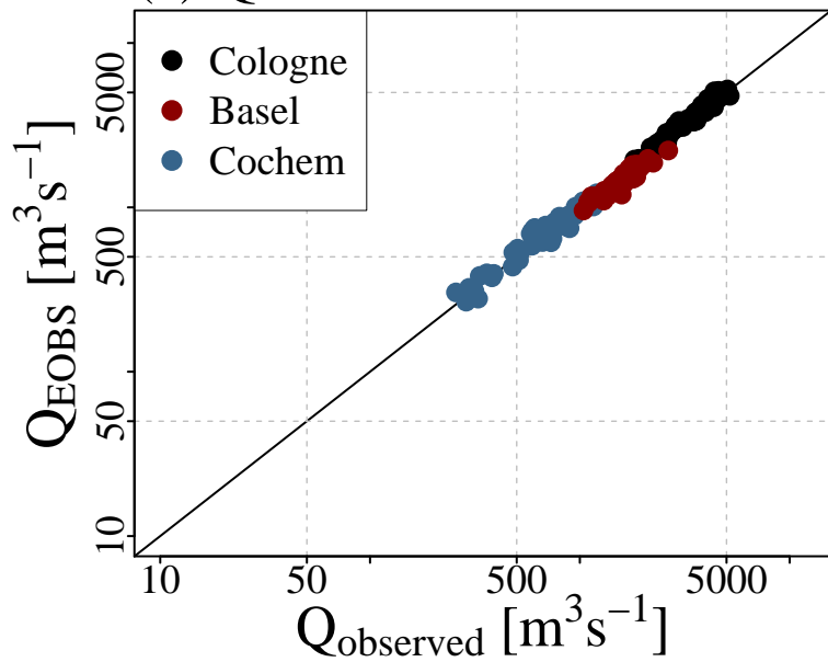
(e) Q90 Observed vs. EOBS
