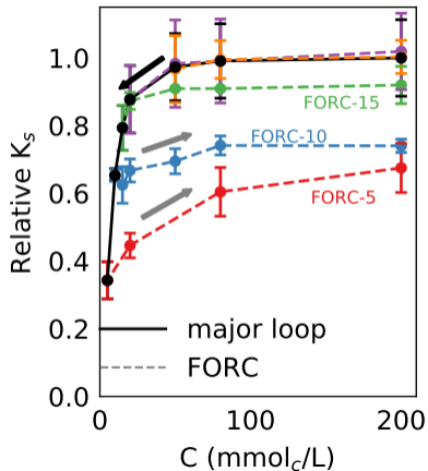
(a) Measured FORCs
