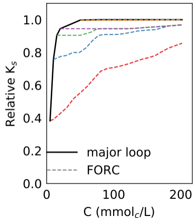
(c) Modeled FORCs
