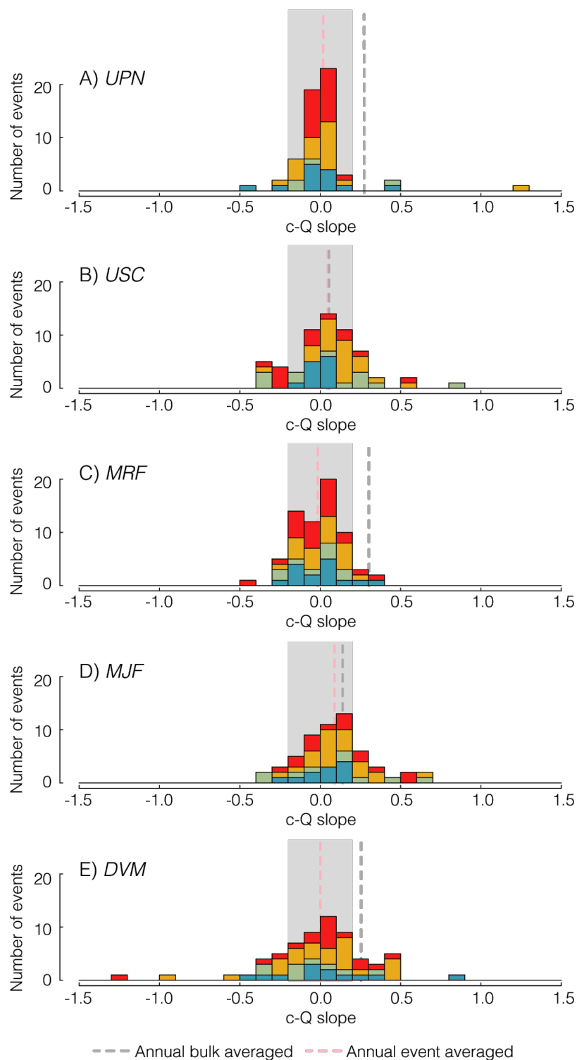
Figure S4 Histograms of individual event c-Q slope for each watershed colored by season. Gray dashed line shows the bulk stormflow c-Q slope and the pink dashed line shows the event-averaged c-Q slope. Gray boxes delineate chemostatic behavior ( |c-Q \text{ slope}| < 0.2 ).
