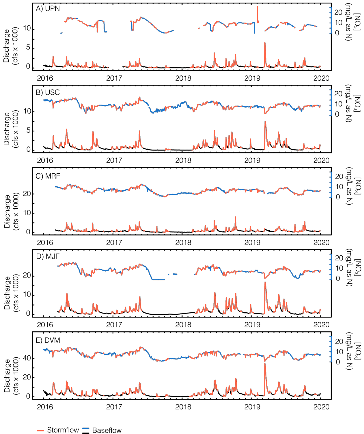
Figure S1 Paired hydrographs and chemographs for the 5 study watersheds with identified events shown in red and baseflow shown in black (hydrograph) and blue (chemograph). Events were identified using the hydrograph, see section 2.3 for details. The record begins in January 2016 and ends in December 2019.
