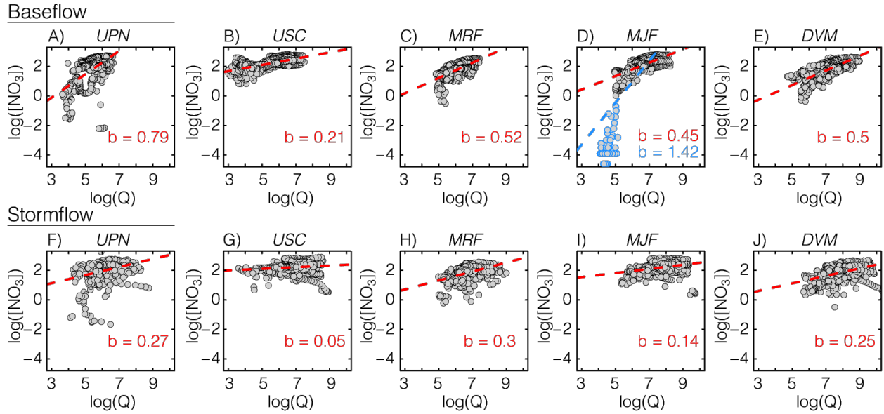
Figure S3 Concentration-discharge plots shown on log-log axes for five studied watersheds during baseflow (A-E) and stormflow (F-J), with the slope shown in red. Panel D shows the baseflow for MJF with the low flow period from 7/27/17-10/19/17 when [\text{NO}_3^-] < 0.5 \text{ mg/L} included (blue) and excluded (red). All slopes are statistically significant ( p < 0.01 )
