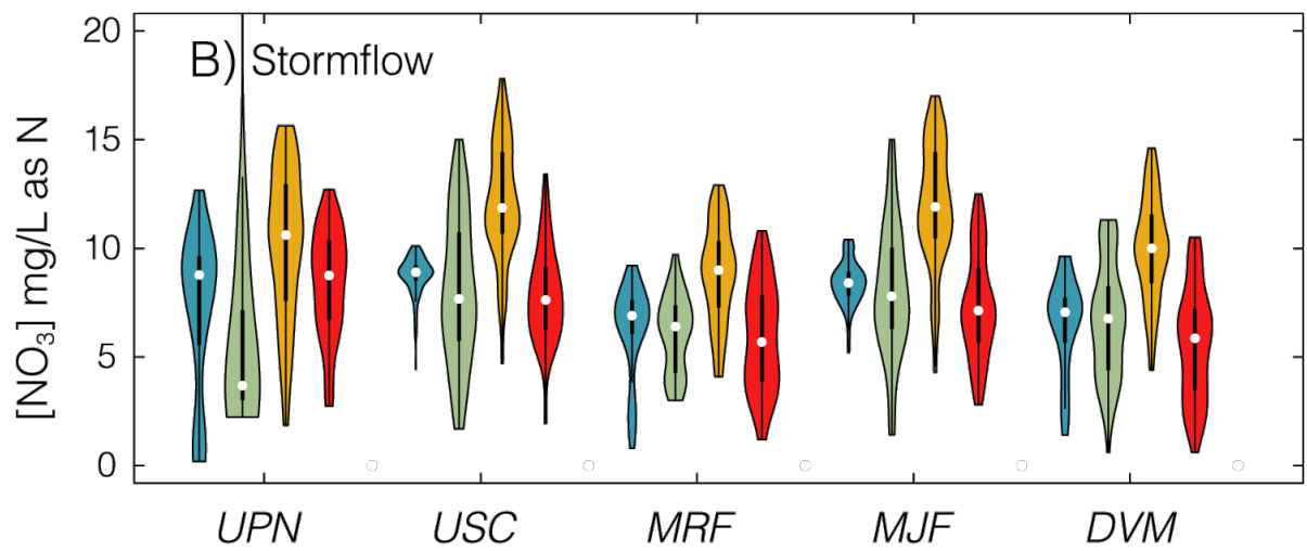
Figure S2 NO 3 - concentration by season for the five watersheds during baseflow (A) and stormflow periods (B).
