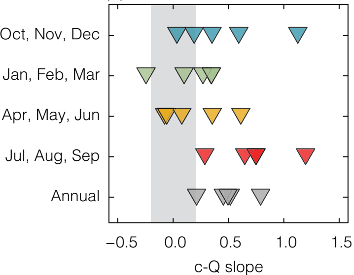
(a) Baseflow
