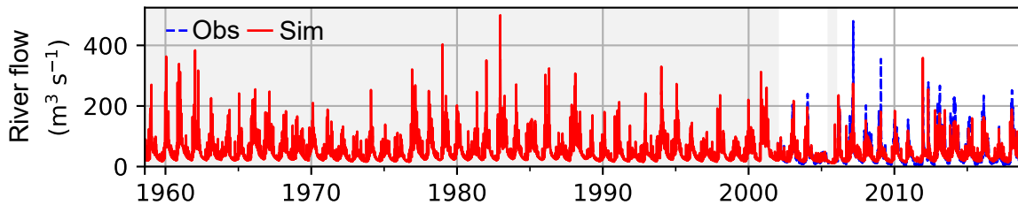
Somme at Abbeville ( E_f = 0.69 , correlation = 0.86, R_d = 0.92 )
