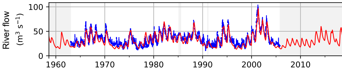
Seine at Poses ( E_f = 0.86 , correlation = 0.93, R_d = 1.02 )
