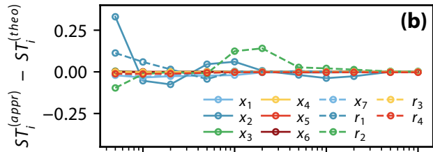
Total Sobol' Index ST_i
