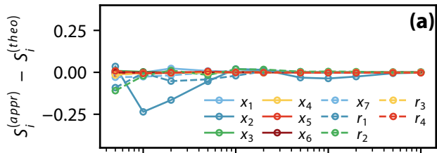
Main Sobol' Index S_i
