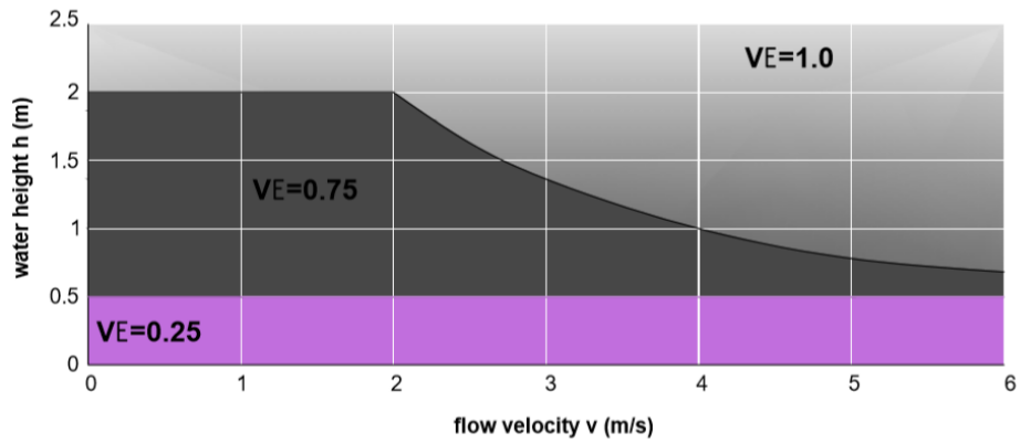
Figure S5: Vulnerability values of the road infrastructure as a function of water height ( h ) and flow velocity ( v ) as proposed in the ISPRA 2012) guidelines
