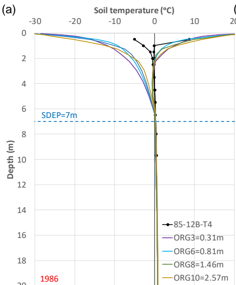
JMR – ORG (TBOT=+0.8°C)
