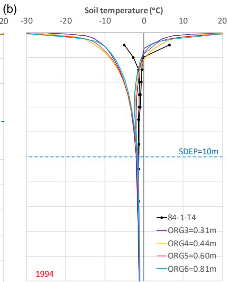
BWC – ORG (TBOT=-1°C)
