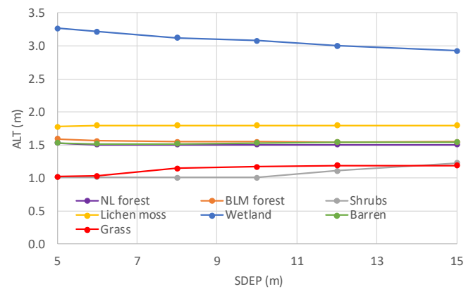
HPC – NL forest (org 0.60m, TBOT=-1.5°C)
