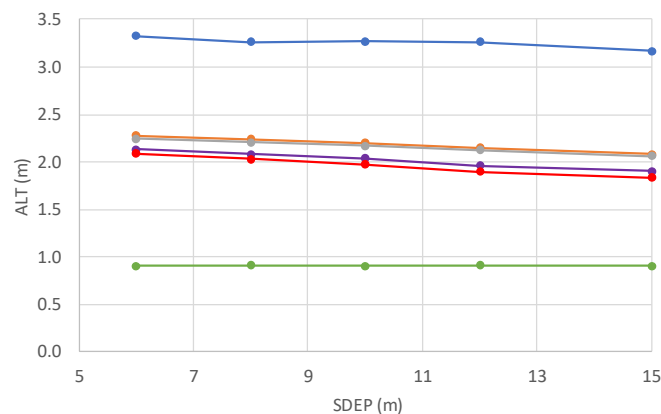
BWC – NL forest (ORG 0.44m, TBOT=-1°C)
