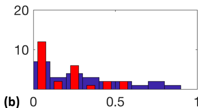
USGS gauge exp. – clim. initial condition
