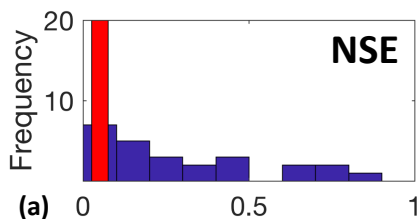
USGS gauge exp. – null initial condition
