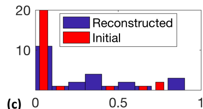
USGS gauge exp. – TMPA initial condition
