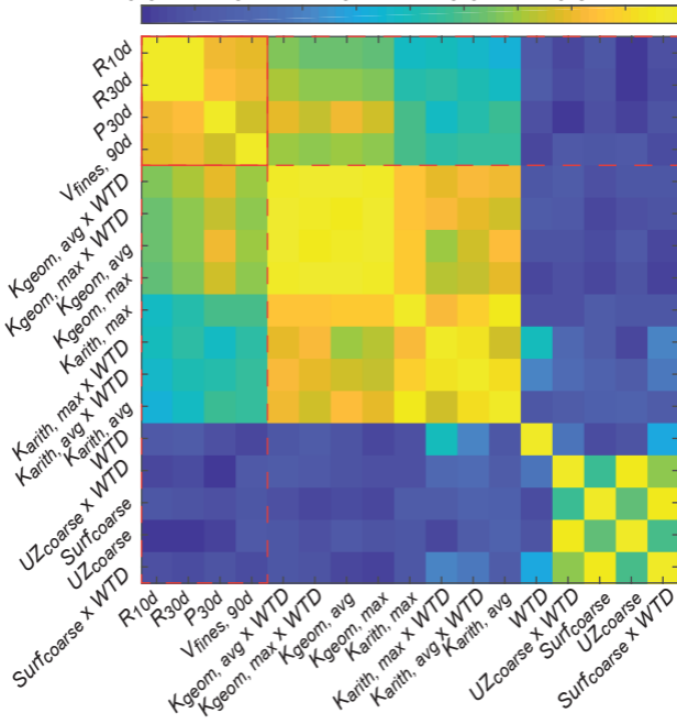
Correlation (absolute value of Pearson's r )
